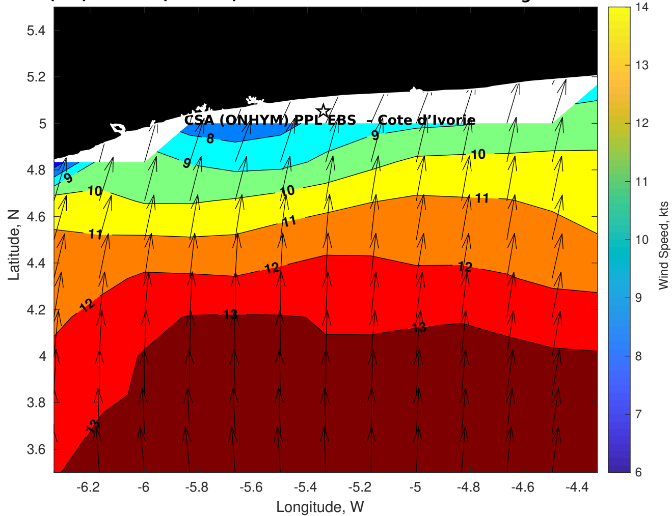
Winds (kts) for CSA (ONHYM) PPL EBS - Cote d'Ivoire at 18-Aug-2025 09:00:00
