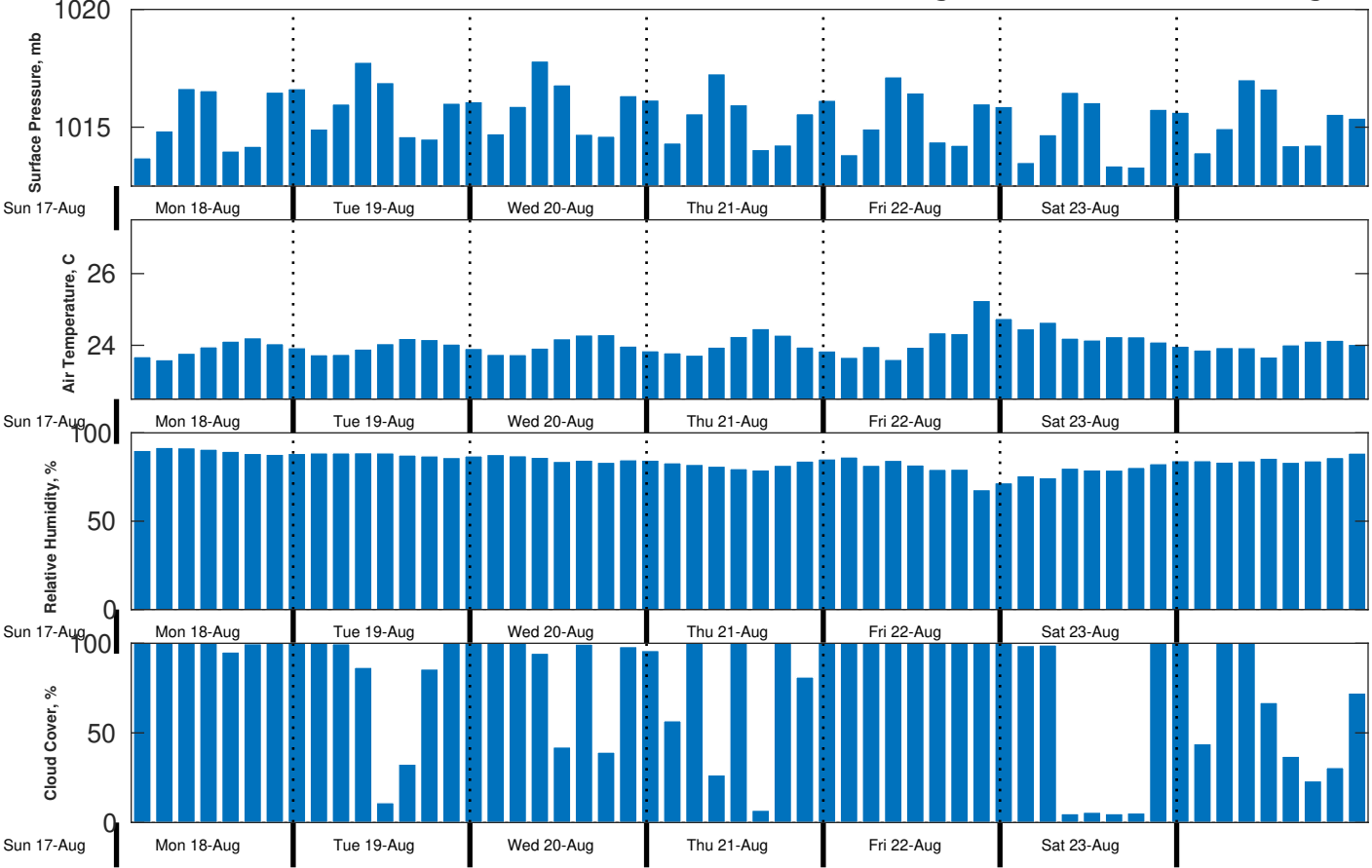
Met Forecast for CSA (ONHYM) PPL EBS - Cote d'Ivoire from 18-Aug-2025 00:00:00 to 25-Aug-2025 00:00:00
