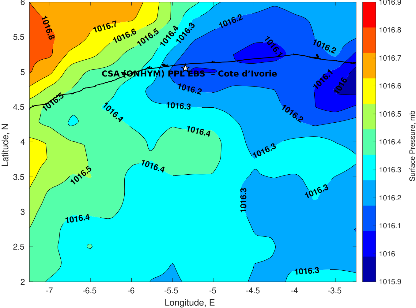
Surface Pressure (mb) for CSA (ONHYM) PPL EBS - Cote d'Ivoire at 20-Aug-2025 00:00:00
