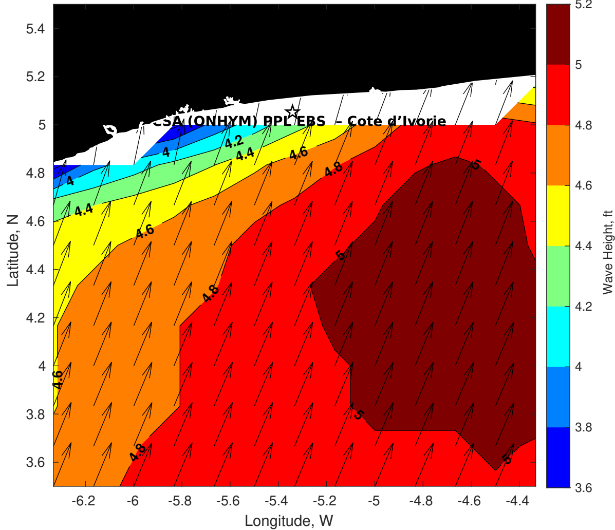
Wave Height (ft) for CSA (ONHYM) PPL EBS - Cote d'Ivoire at 18-Aug-2025 09:00:00
