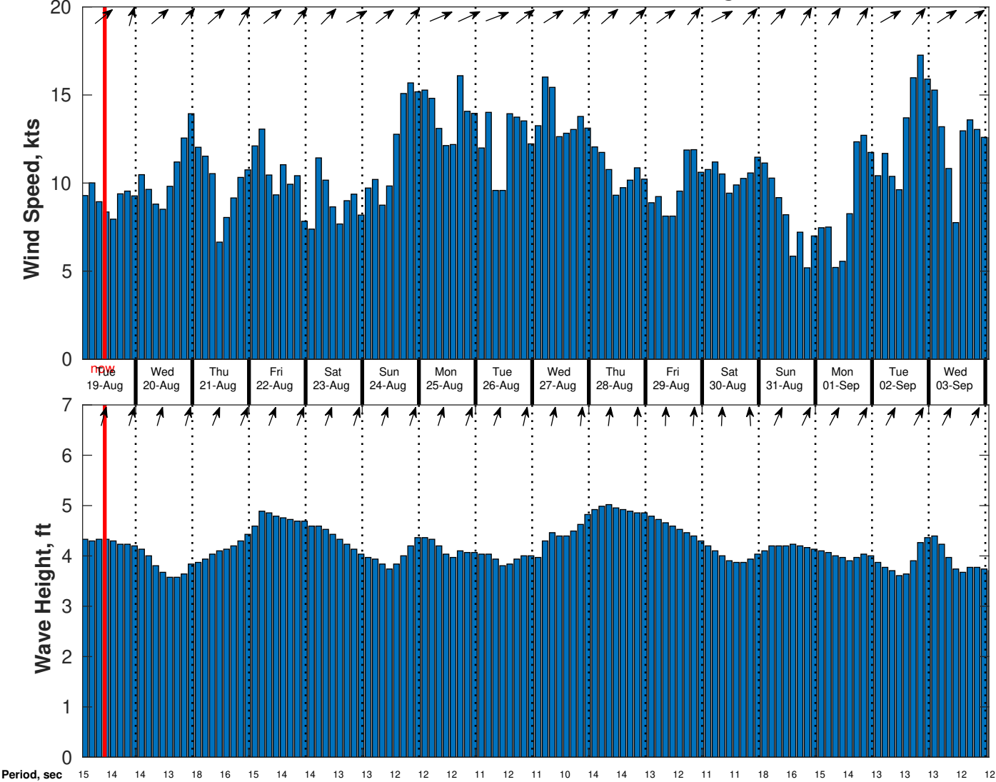
Wind & Wave Forecast for CSA (ONHYM) PPL EBS - Cote d'Ivoire from 18-Aug-2025 01:00:00 to 03-Sep-2025 01:00:00
