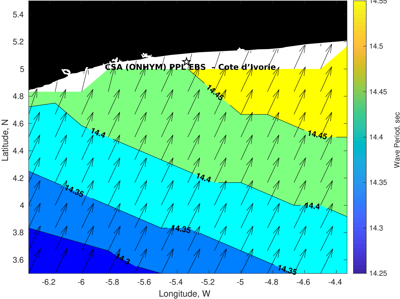
Wave Period (sec) for CSA (ONHYM) PPL EBS - Cote d'Ivoire at 18-Aug-2025 09:00:00
