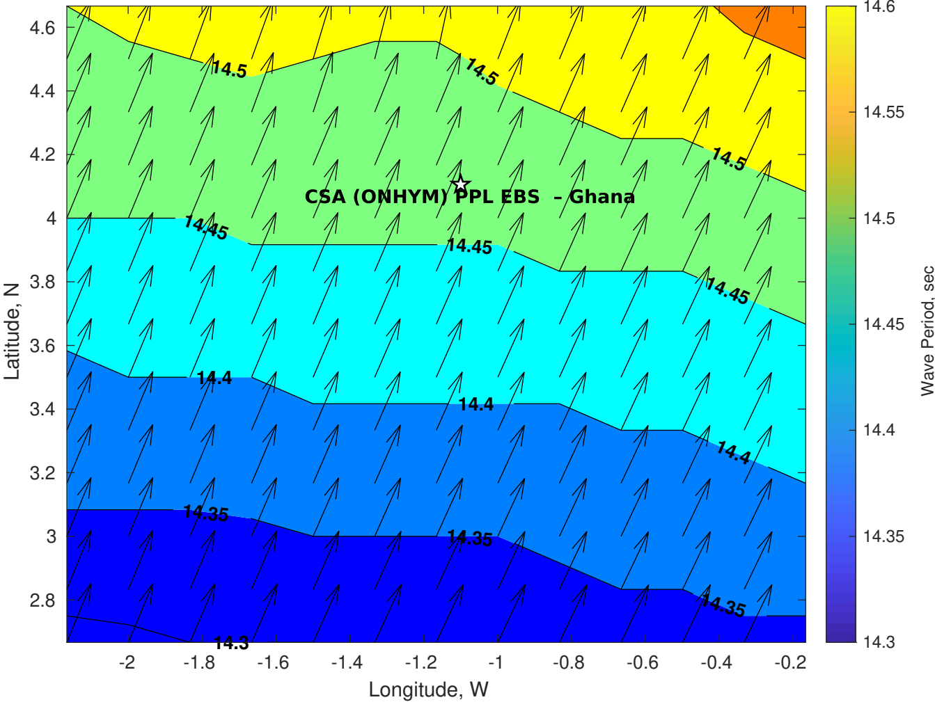
Wave Period (sec) for CSA (ONHYM) PPL EBS - Ghana at 18-Aug-2025 09:00:00
