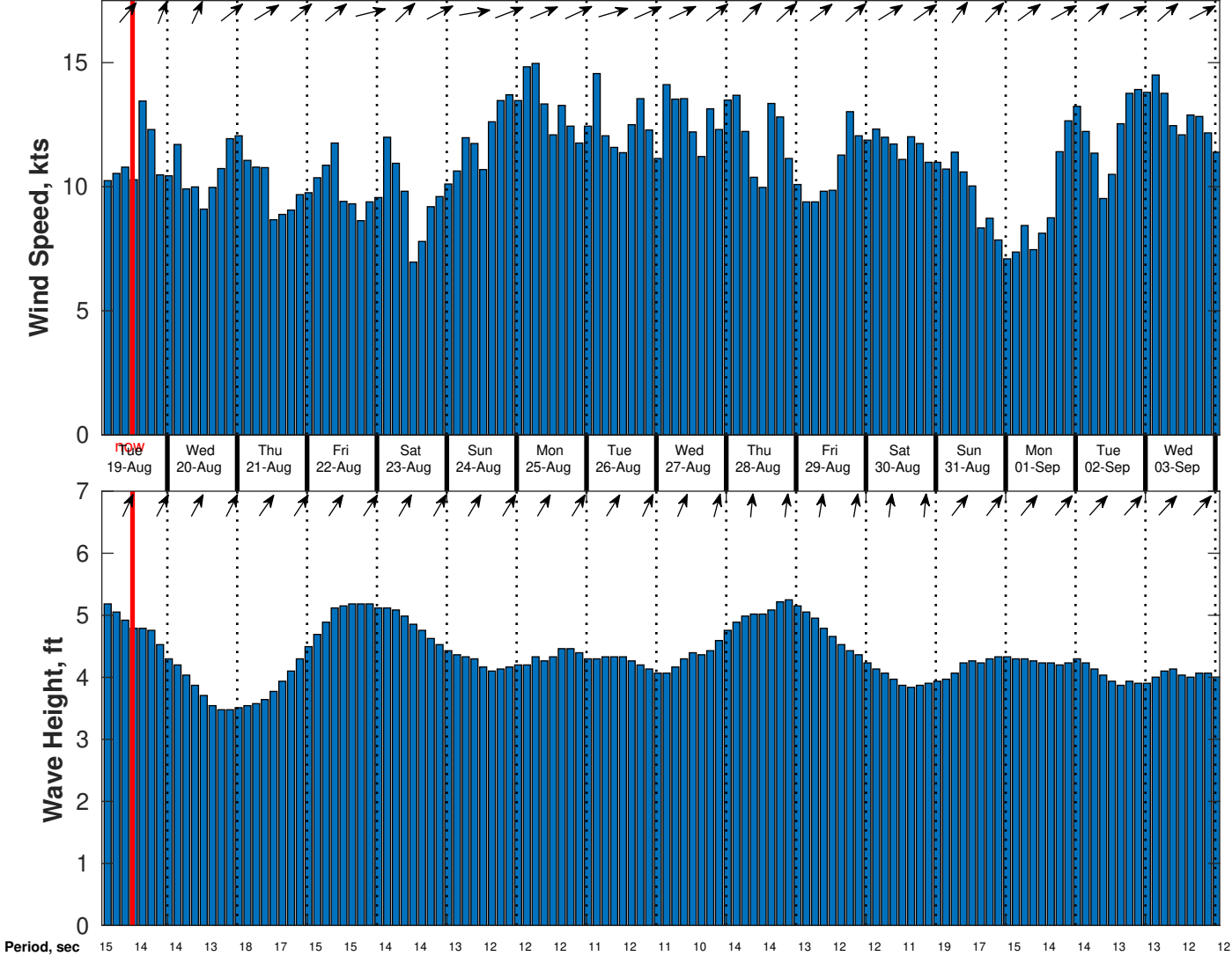
Wind & Wave Forecast for CSA (ONHYM) PPL EBS - Ghana from 18-Aug-2025 02:00:00 to 03-Sep-2025 02:00:00
