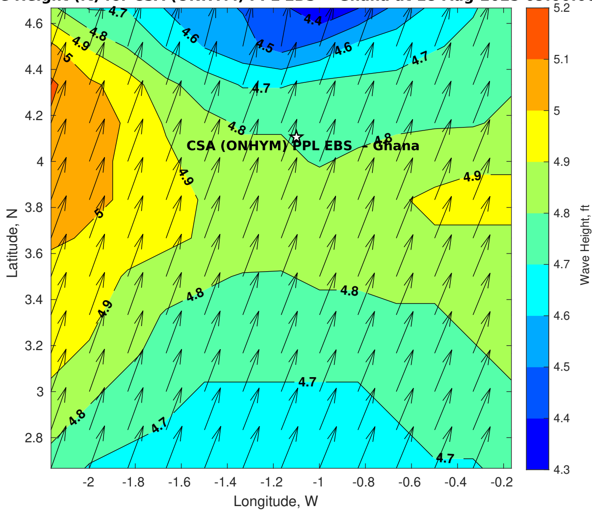
Wave Height (ft) for CSA (ONHYM) PPL EBS - Ghana at 18-Aug-2025 09:00:00
