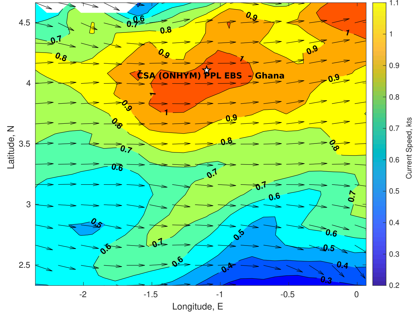
Surface Currents for CSA (ONHYM) PPL EBS - Ghana at 17-Aug-2025 00:00:00
