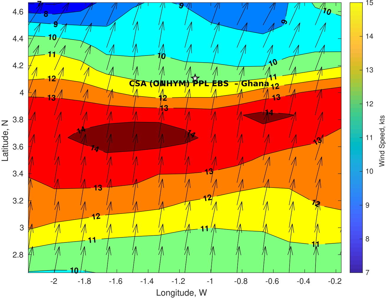
Winds (kts) for CSA (ONHYM) PPL EBS - Ghana at 18-Aug-2025 09:00:00
