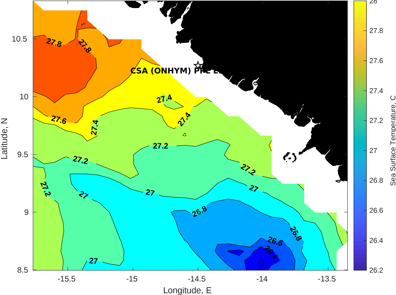
SST for CSA (ONHYM) PPL EBS - Guinea at 17-Aug-2025 00:00:00
