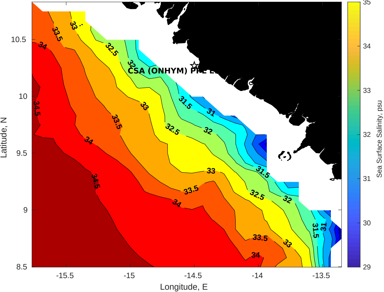
Surface Salinity for CSA (ONHYM) PPL EBS - Guinea at 17-Aug-2025 00:00:00
