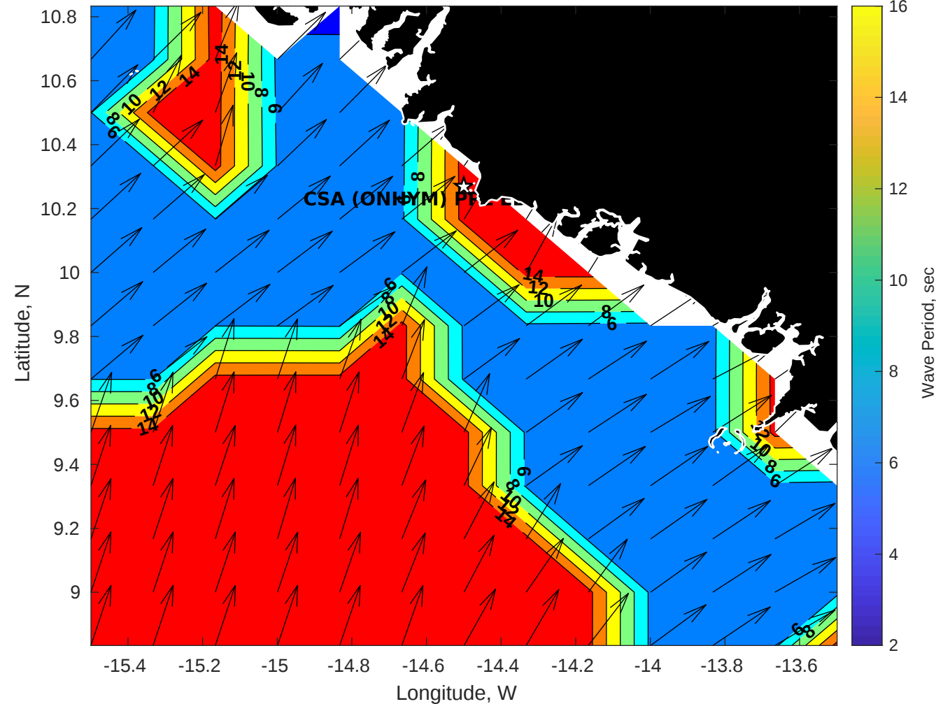
Wave Period (sec) for CSA (ONHYM) PPL EBS - Guinea at 18-Aug-2025 09:00:00
