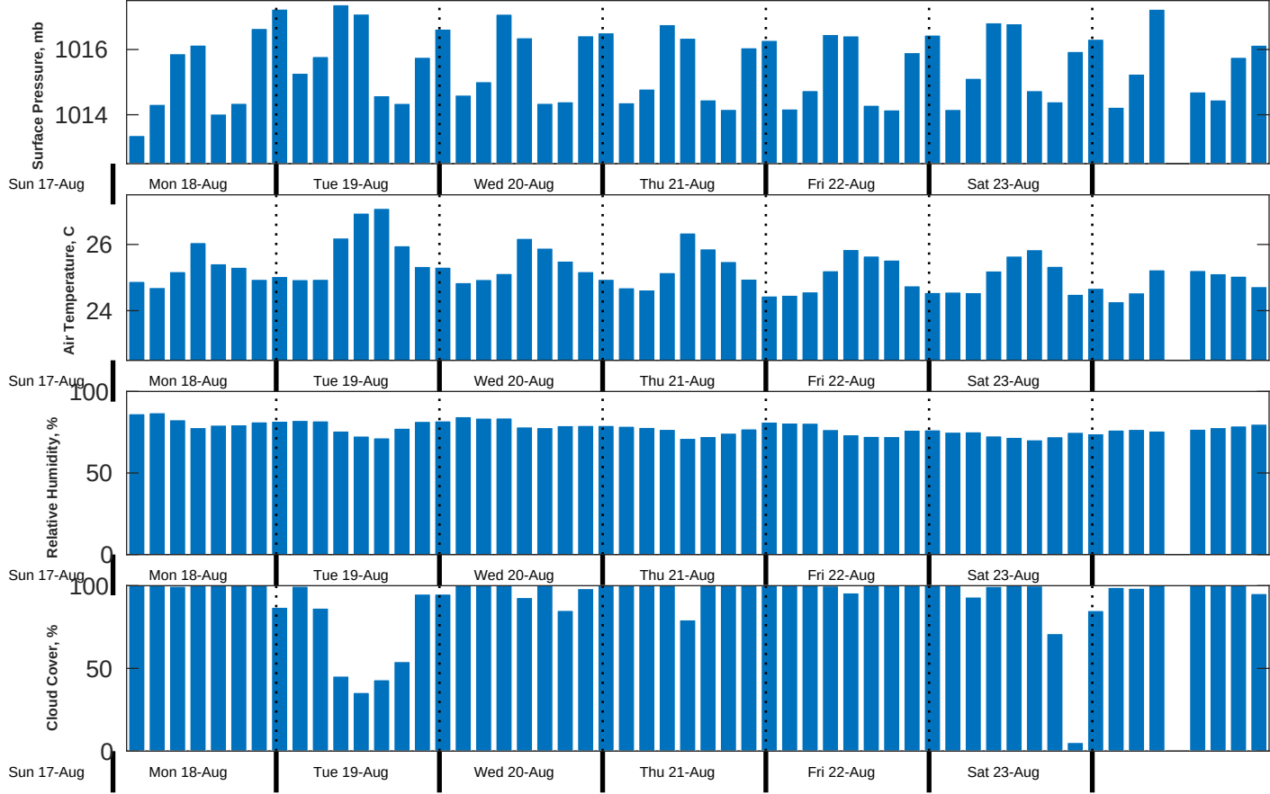
Met Forecast for CSA (ONHYM) PPL EBS - Liberia from 18-Aug-2025 00:00:00 to 25-Aug-2025 00:00:00
