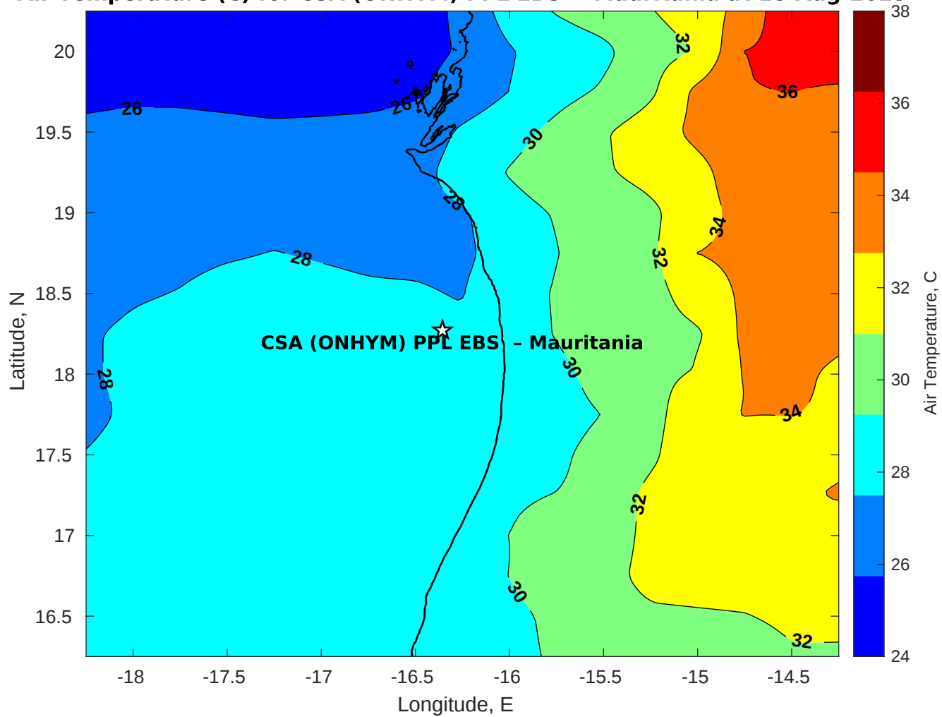
Air Temperature (C) for CSA (ONHYM) PPL EBS - Mauritania at 18-Aug-2025
