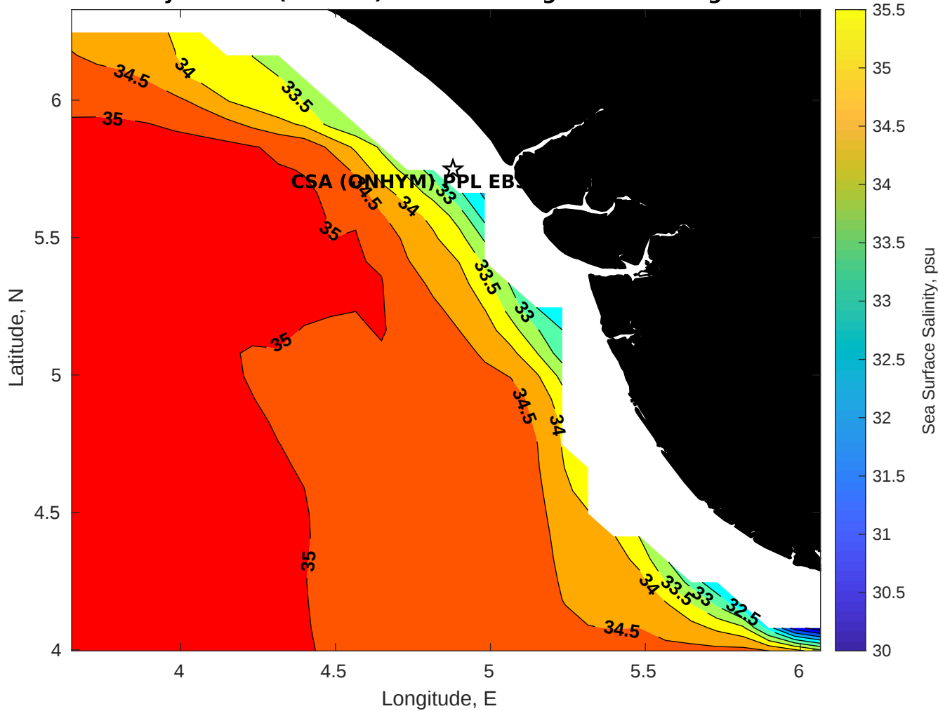
Surface Salinity for CSA (ONHYM) PPL EBS - Nigeria at 17-Aug-2025 00:00:00
