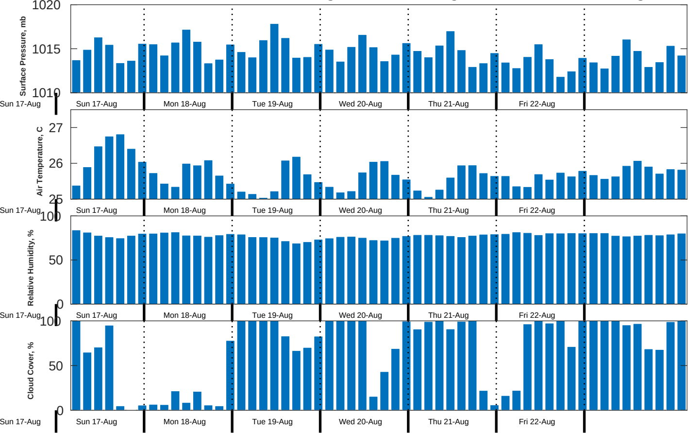
Met Forecast for CSA (ONHYM) PPL EBS - Nigeria from 18-Aug-2025 00:00:00 to 25-Aug-2025 00:00:00
