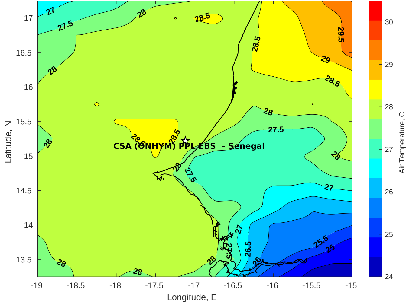
Air Temperature (C) for CSA (ONHYM) PPL EBS - Senegal at 18-Aug-2025
