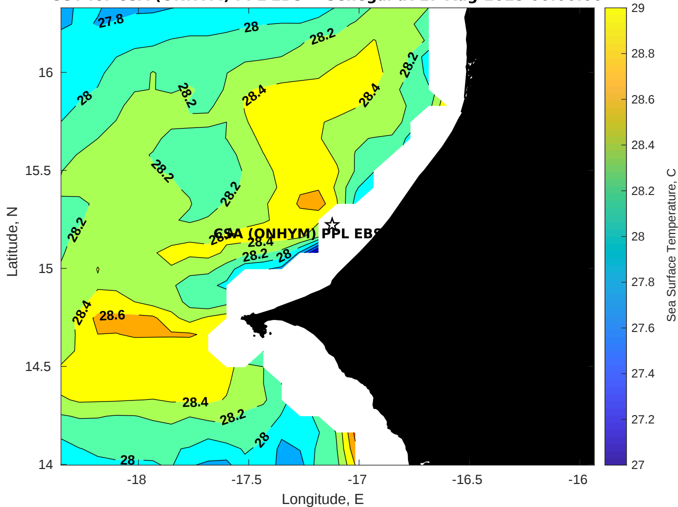
SST for CSA (ONHYM) PPL EBS - Senegal at 17-Aug-2025 00:00:00
