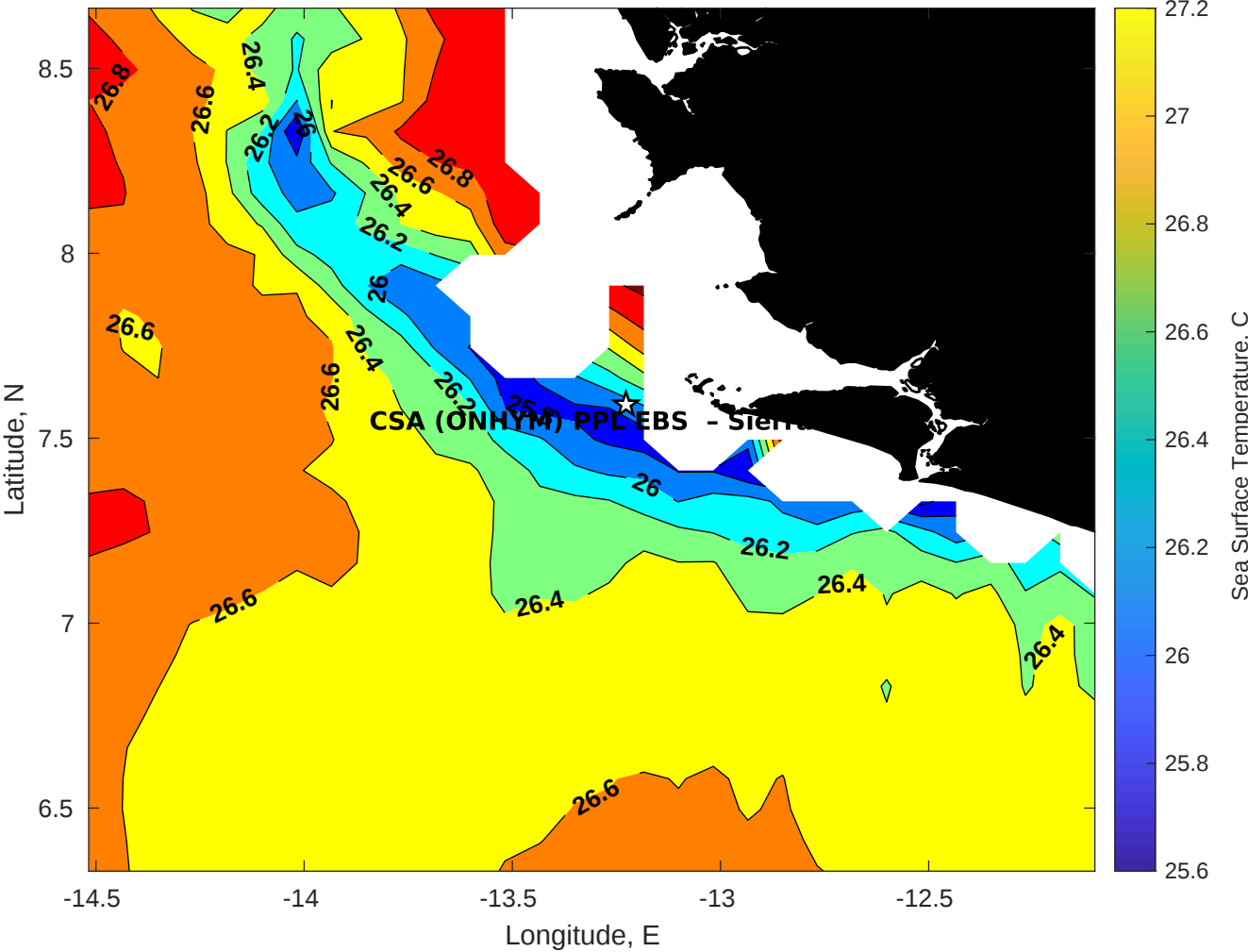
SST for CSA (ONHYM) PPL EBS - Sierra Leone at 17-Aug-2025 00:00:00
