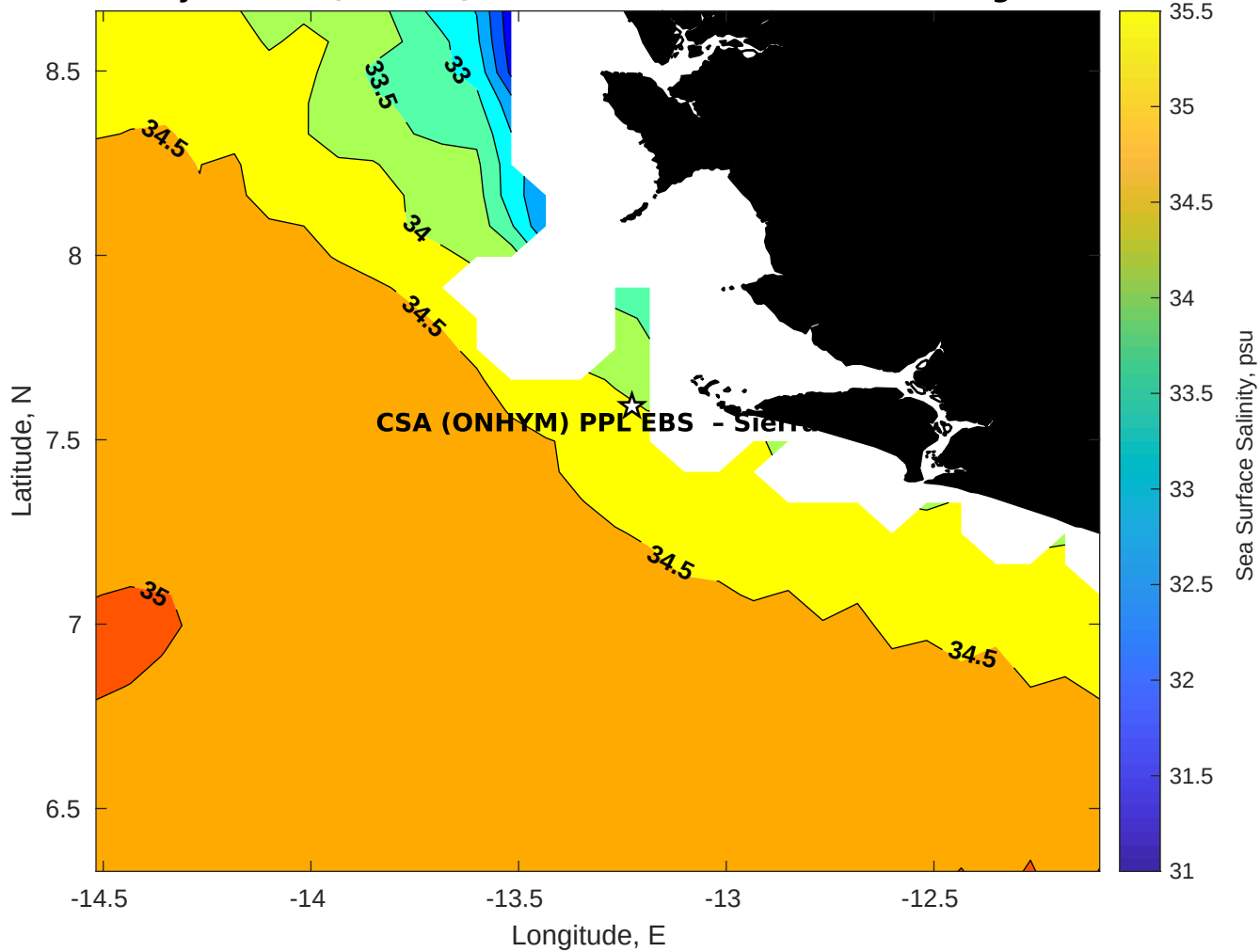
Surface Salinity for CSA (ONHYM) PPL EBS - Sierra Leone at 17-Aug-2025 00:00:00
