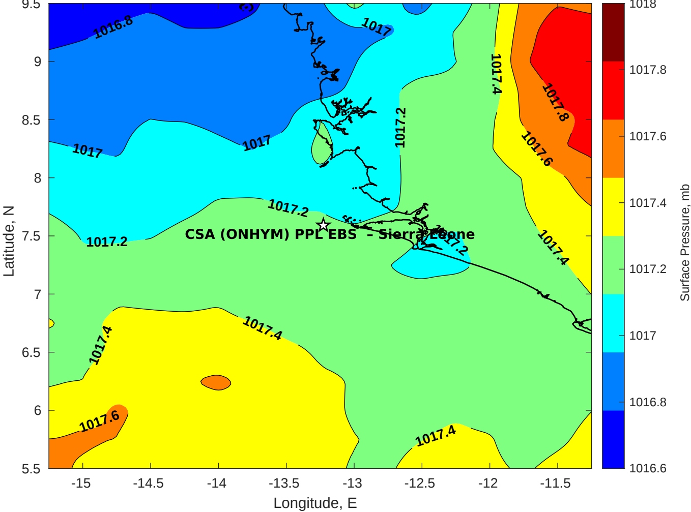
Surface Pressure (mb) for CSA (ONHYM) PPL EBS - Sierra Leone at 19-Aug-2025 00:00:00
