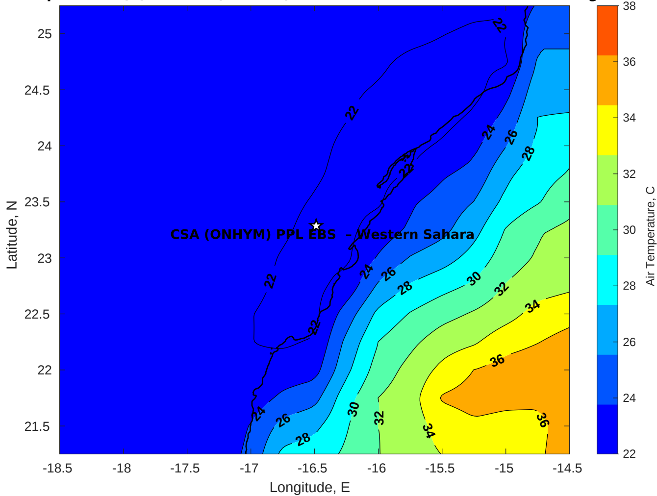
Air Temperature (C) for CSA (ONHYM) PPL EBS - Western Sahara at 18-Aug-2025
