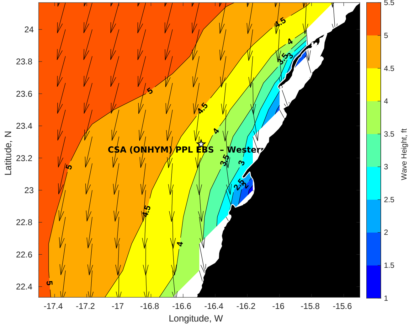
Wave Height (ft) for CSA (ONHYM) PPL EBS - Western Sahara at 18-Aug-2025 09:00:00
