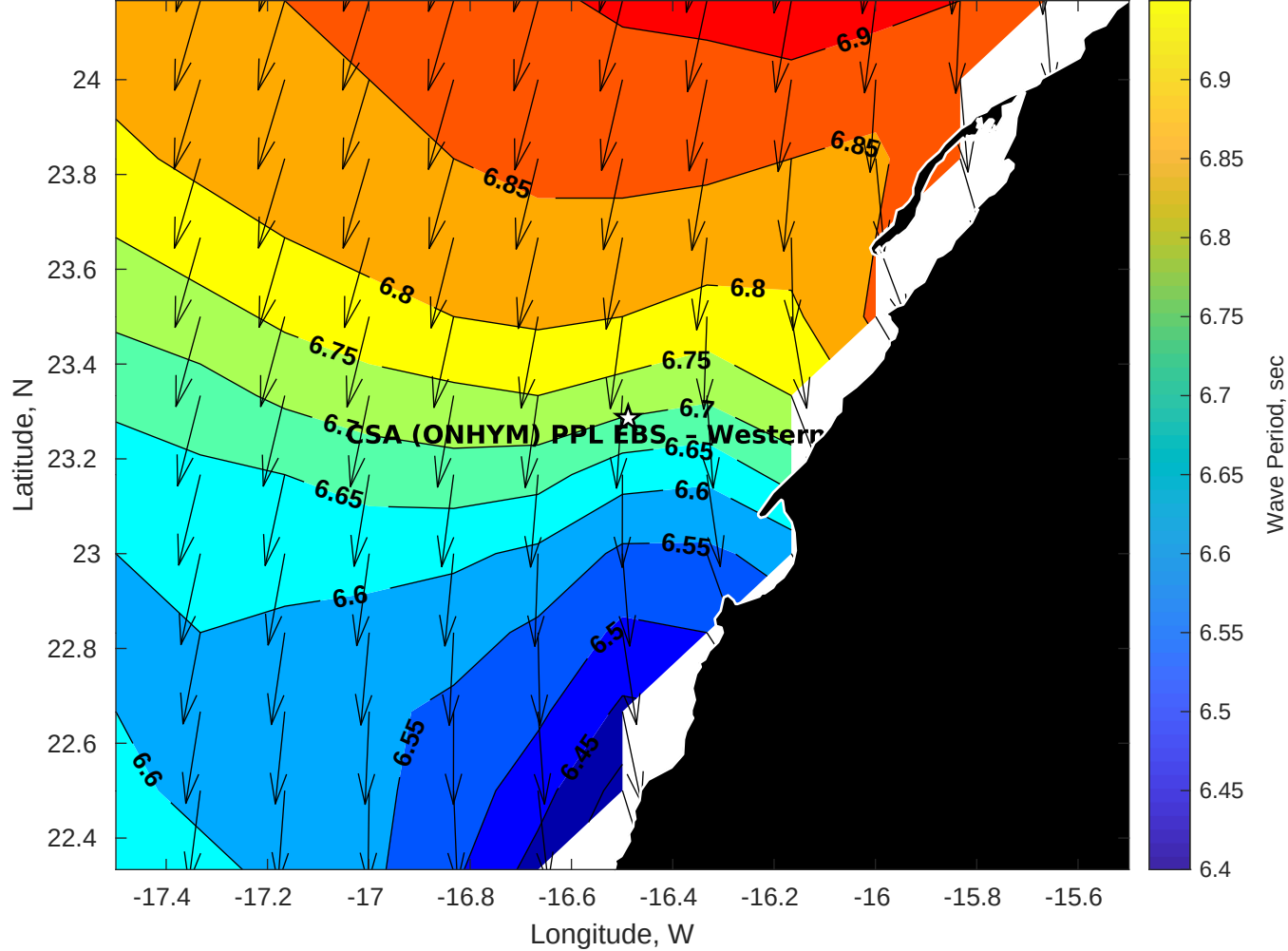
Wave Period (sec) for CSA (ONHYM) PPL EBS - Western Sahara at 18-Aug-2025 09:00:00
