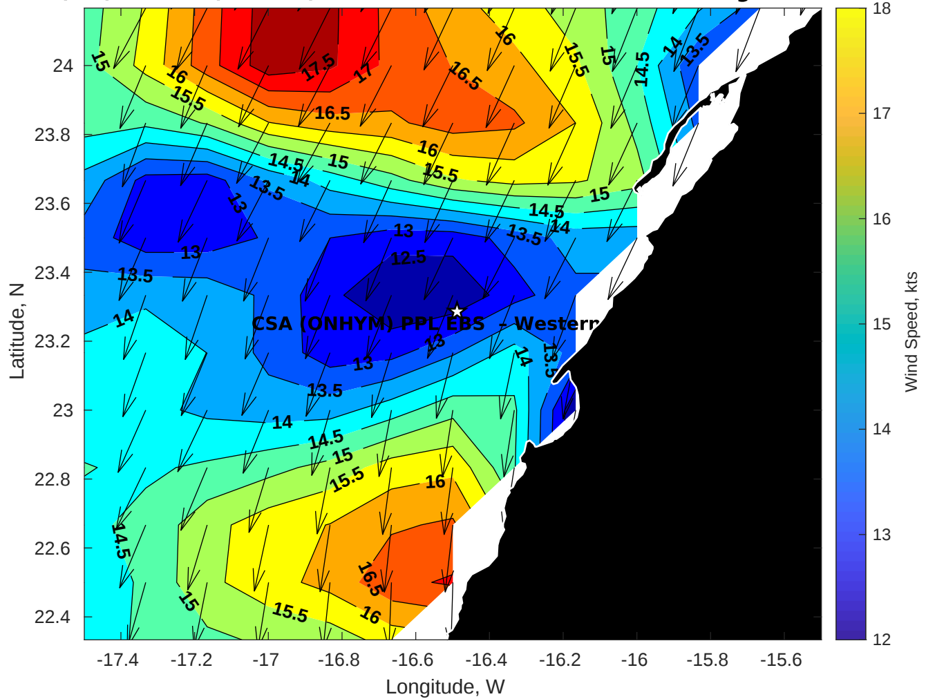
Winds (kts) for CSA (ONHYM) PPL EBS - Western Sahara at 18-Aug-2025 09:00:00
