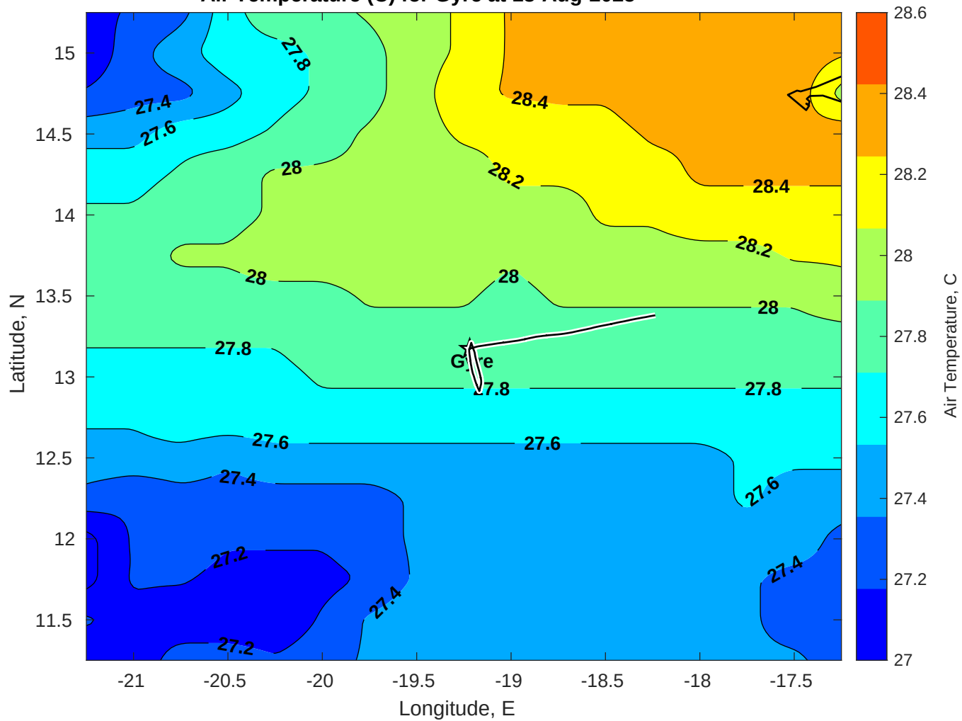
Air Temperature (C) for Gyre at 18-Aug-2025
