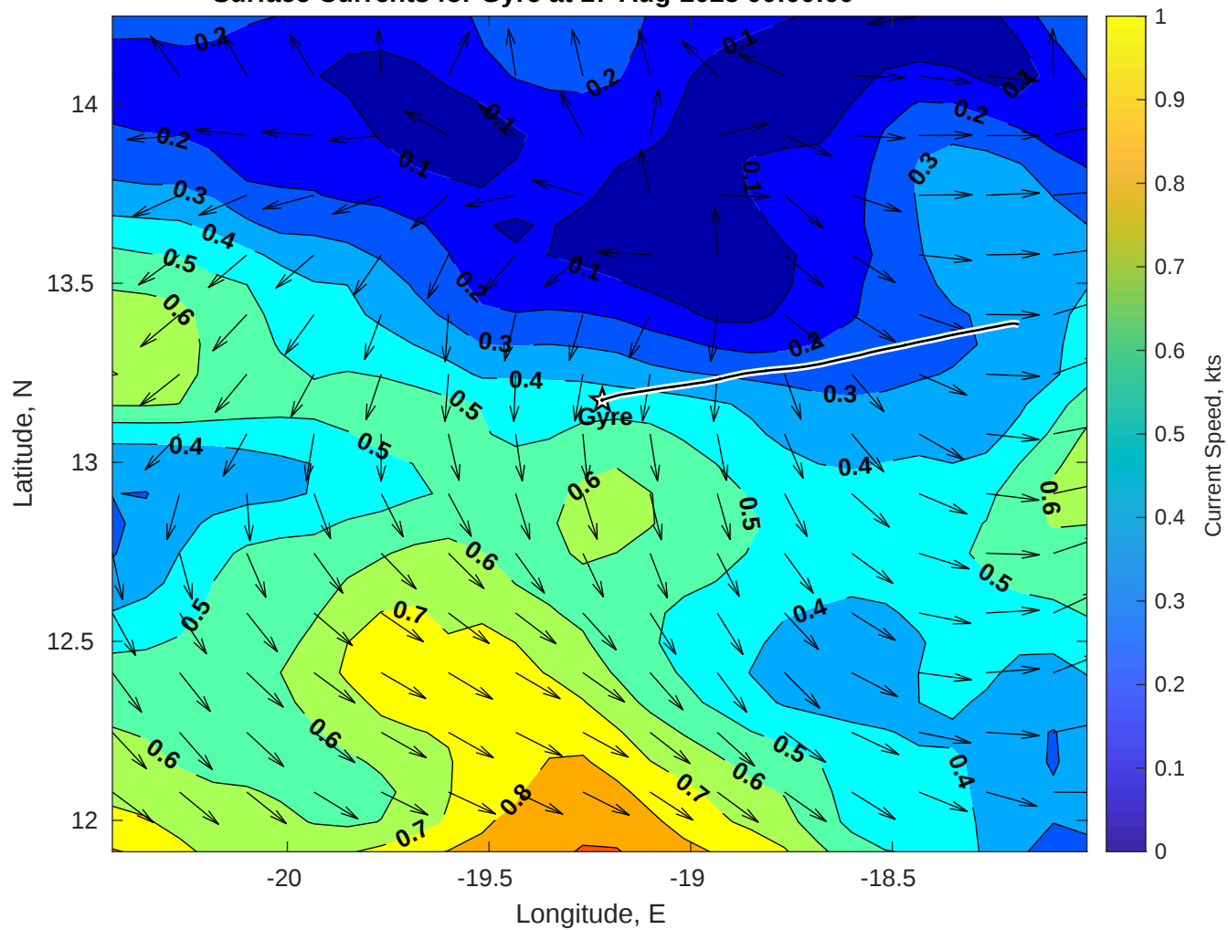
Surface Currents for Gyre at 17-Aug-2025 00:00:00
