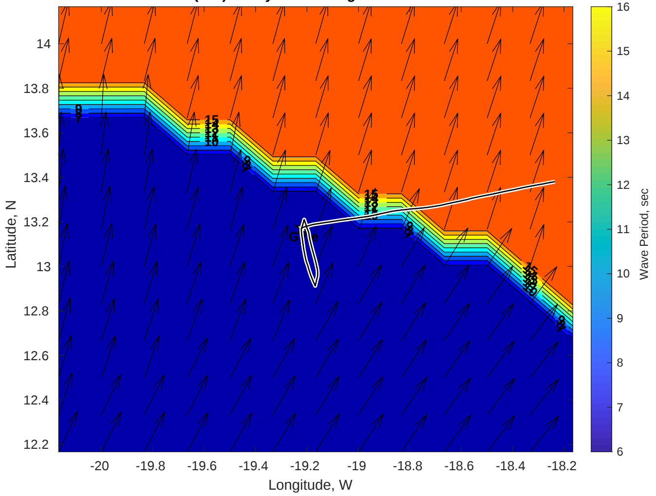
Wave Period (sec) for Gyre at 18-Aug-2025 09:00:00
