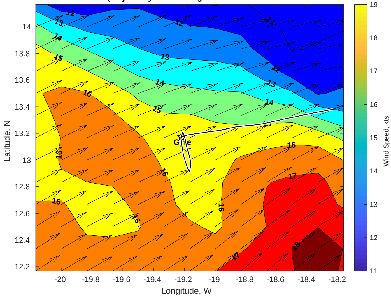
Winds (kts) for Gyre at 18-Aug-2025 09:00:00
