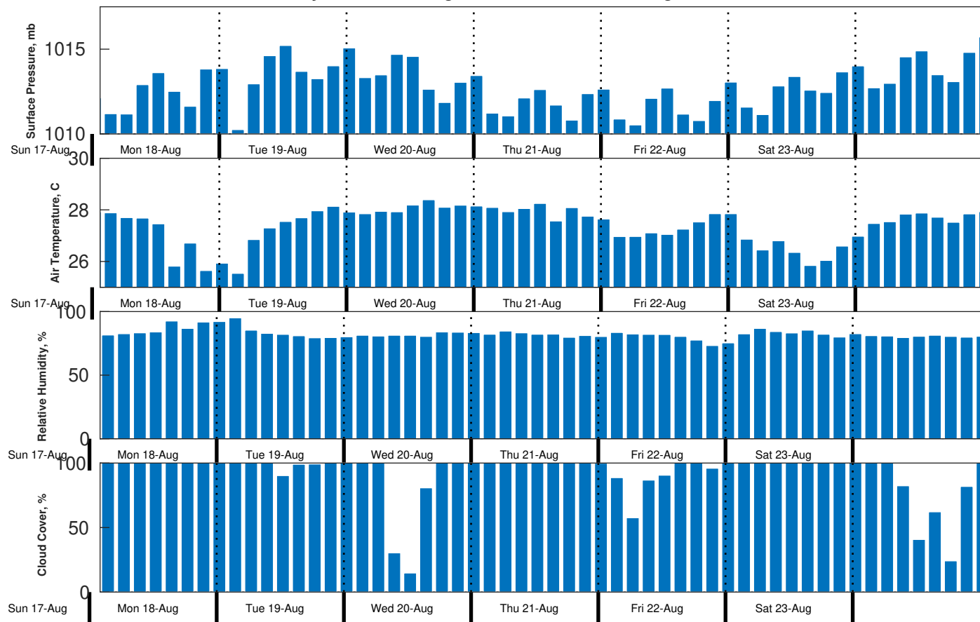
Met Forecast for Gyre from 17-Aug-2025 23:00:00 to 24-Aug-2025 23:00:00
