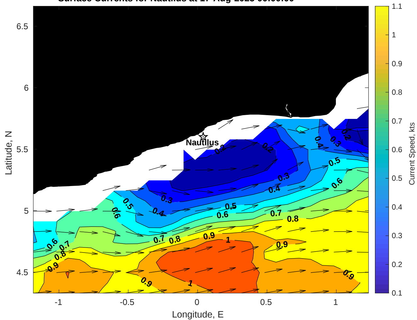
Surface Currents for Nautilus at 17-Aug-2025 00:00:00
