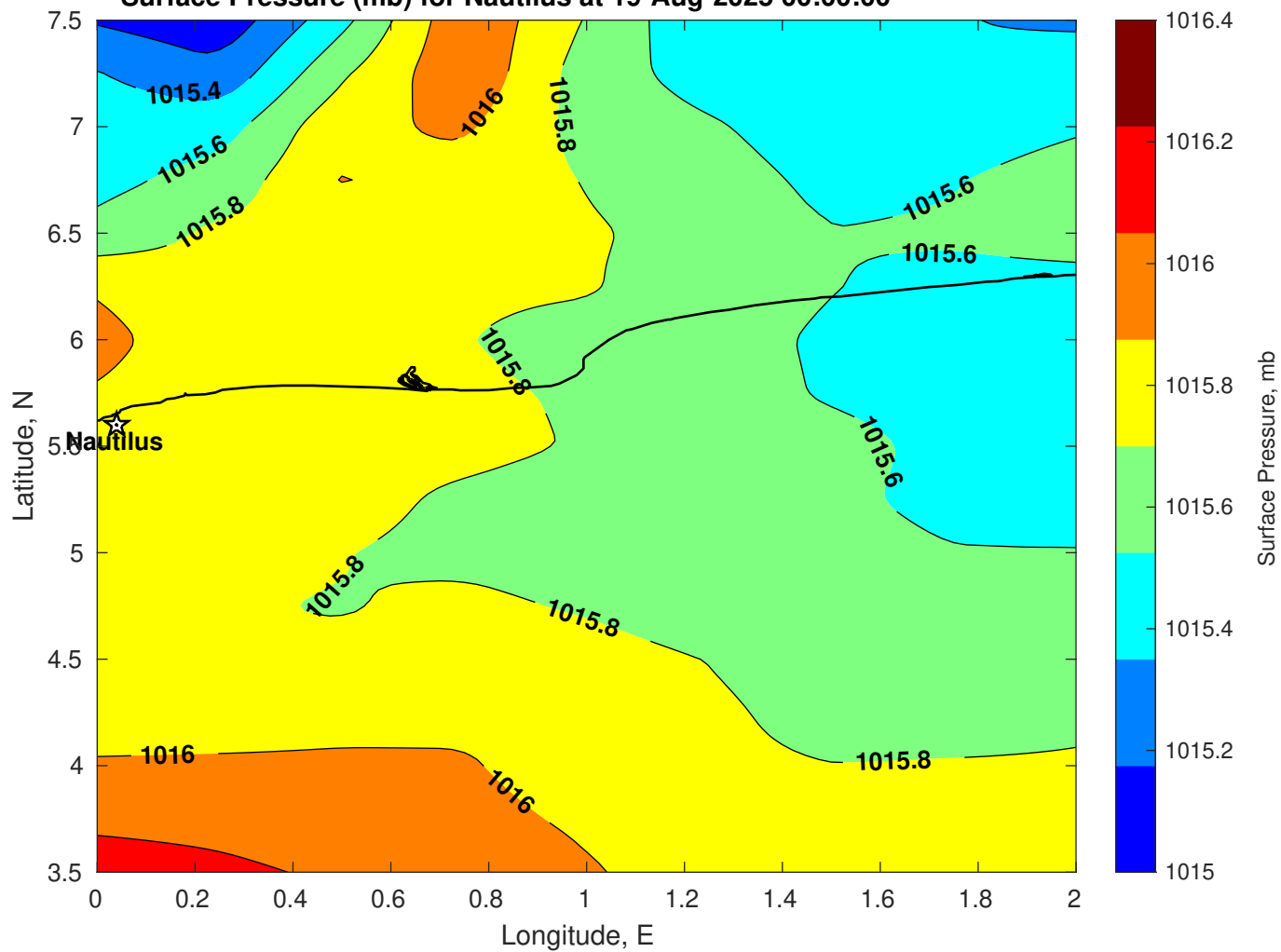
Surface Pressure (mb) for Nautilus at 19-Aug-2025 00:00:00
