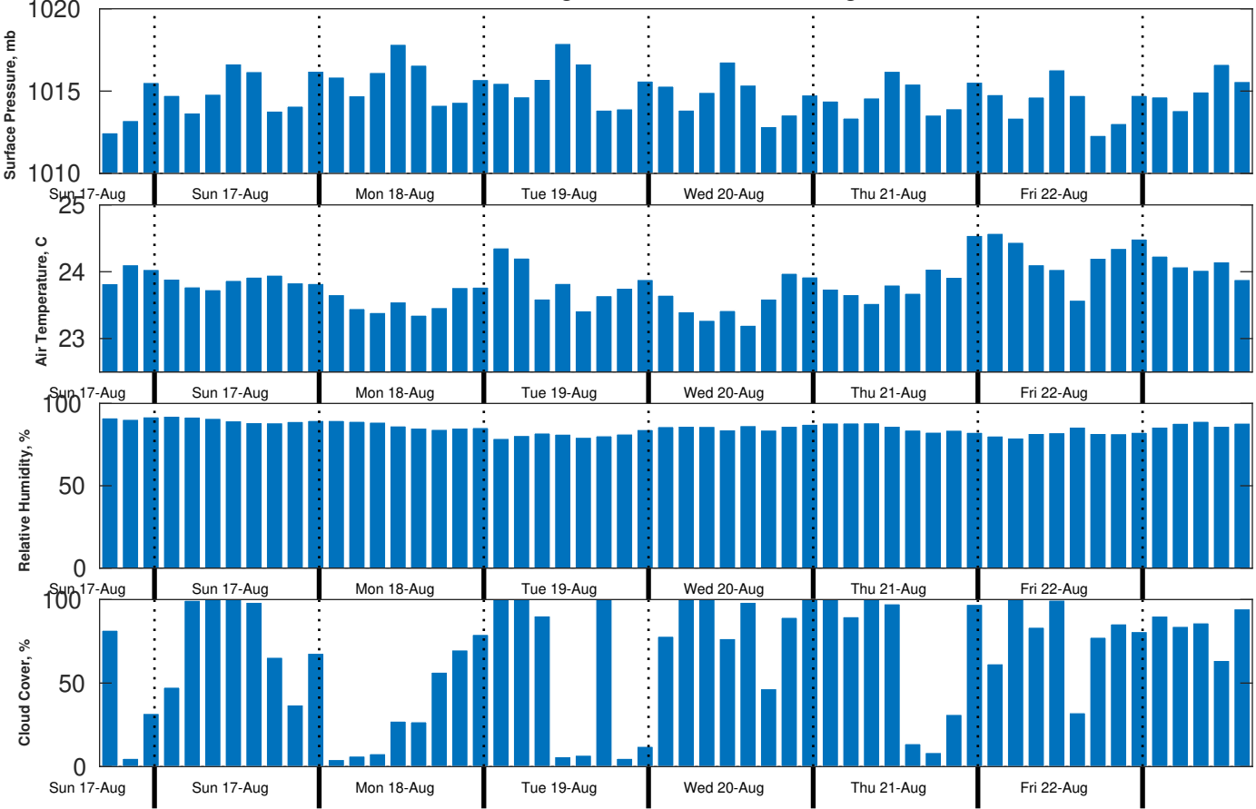
Met Forecast for Nautilus from 17-Aug-2025 12:00:00 to 24-Aug-2025 12:00:00
