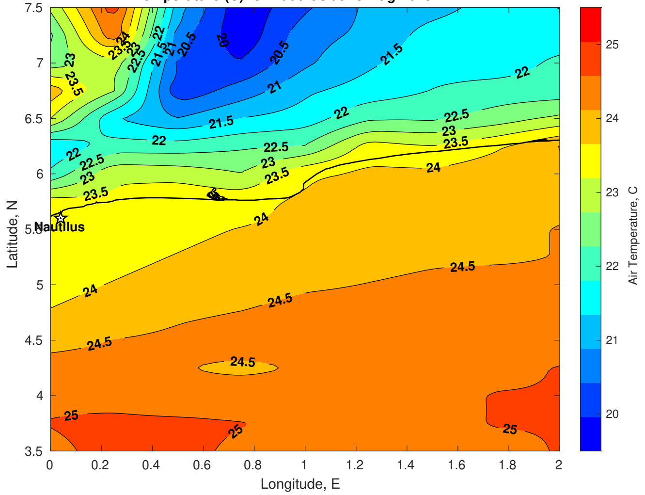
Air Temperature (C) for Nautilus at 18-Aug-2025
