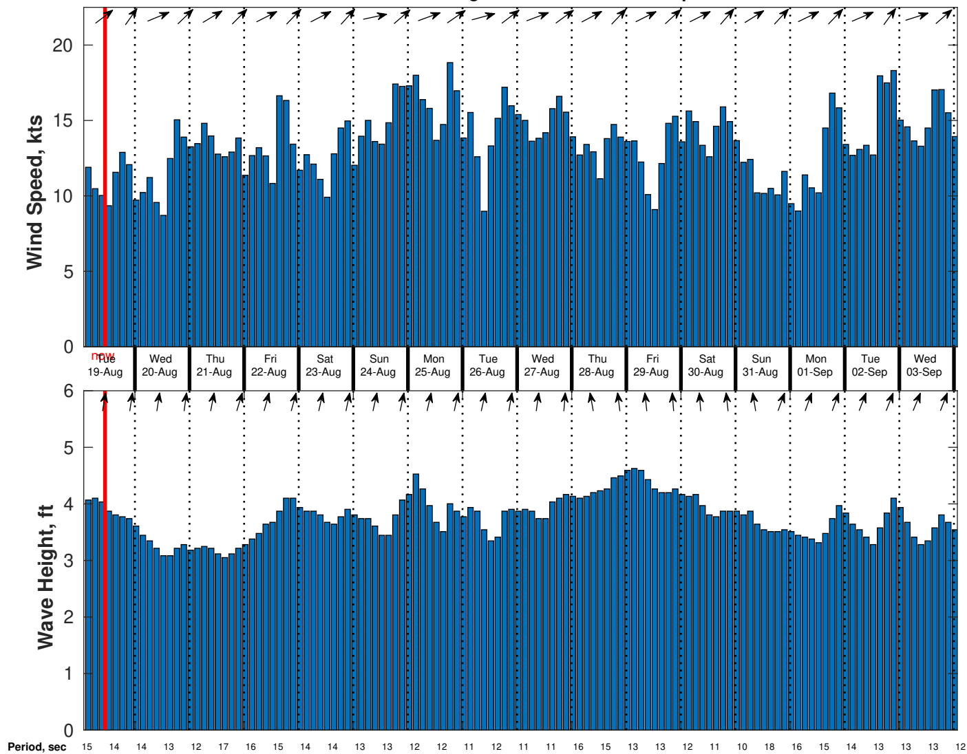
Wind & Wave Forecast for Nautilus from 18-Aug-2025 02:00:00 to 03-Sep-2025 02:00:00
