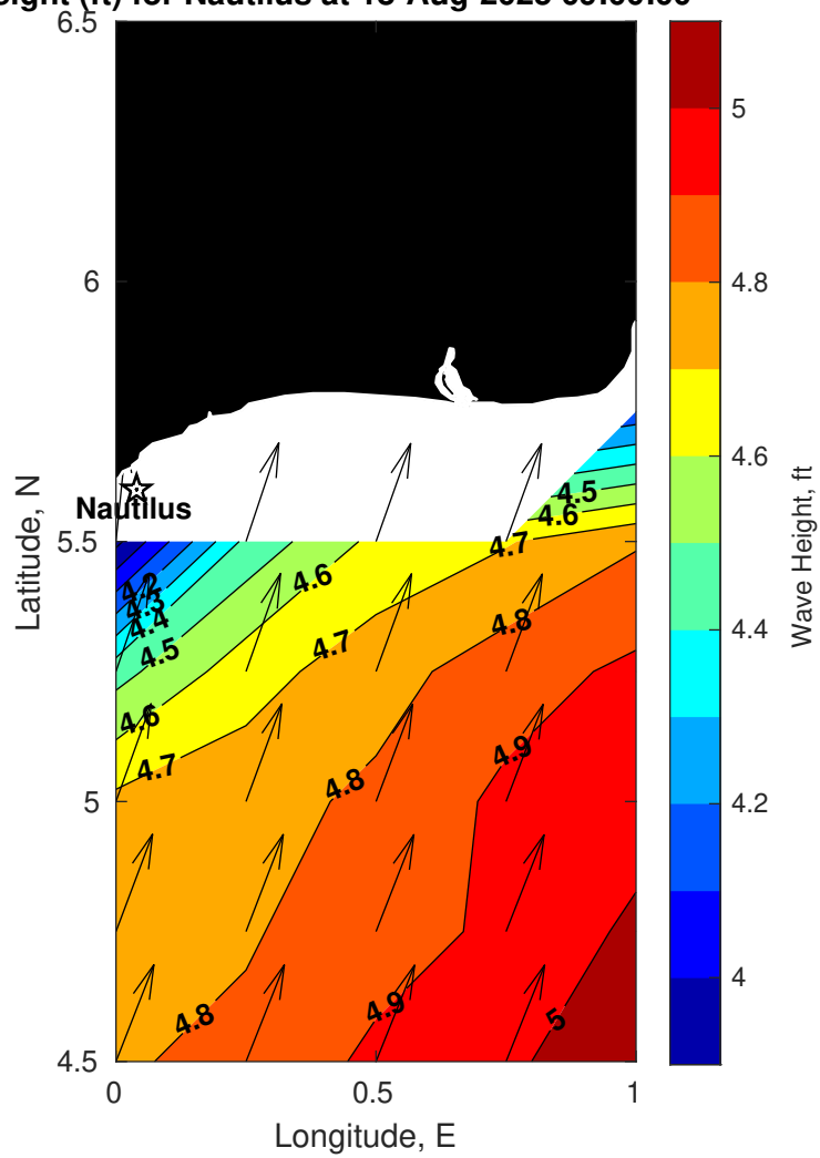
Wave Height (ft) for Nautilus at 18-Aug-2025 09:00:00
