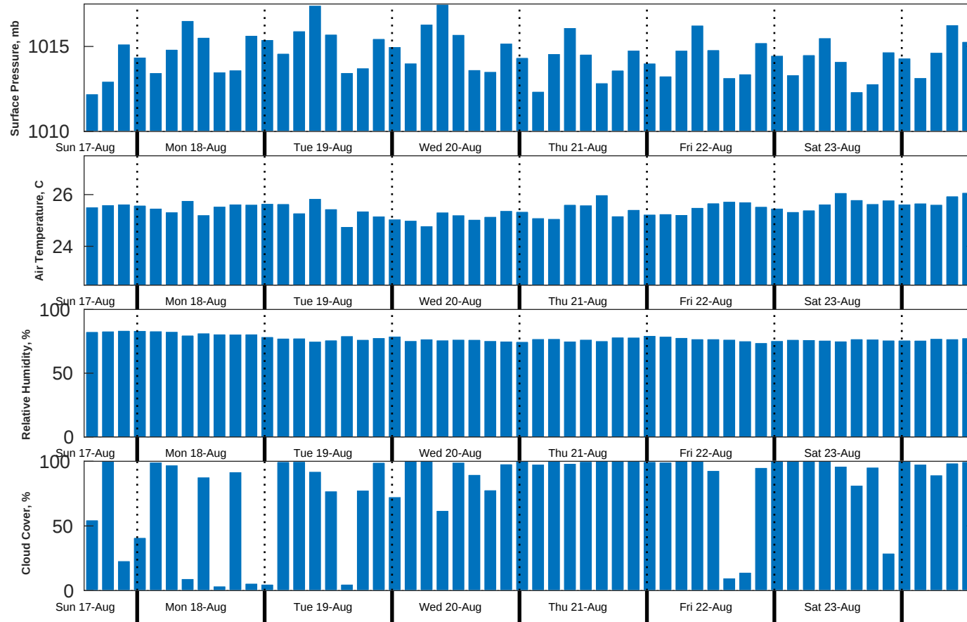
Met Forecast for Proteus from 17-Aug-2025 12:00:00 to 24-Aug-2025 12:00:00
