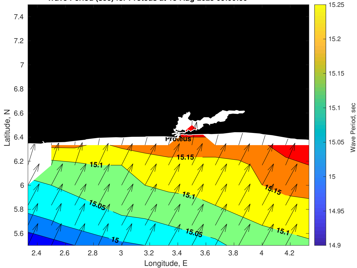
Wave Period (sec) for Proteus at 18-Aug-2025 09:00:00
