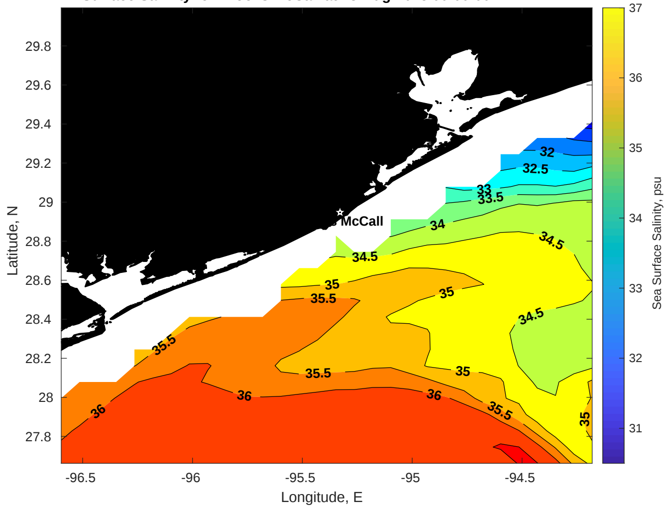
Surface Salinity for Brooks McCall at 18-Aug-2025 00:00:00
