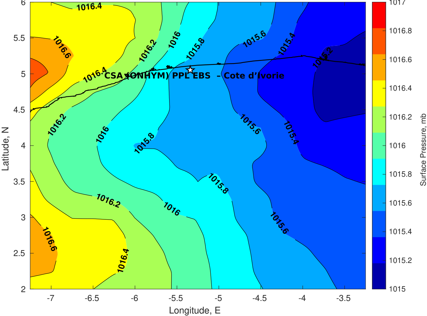
Surface Pressure (mb) for CSA (ONHYM) PPL EBS - Cote d'Ivoire at 21-Aug-2025 00:00:00
