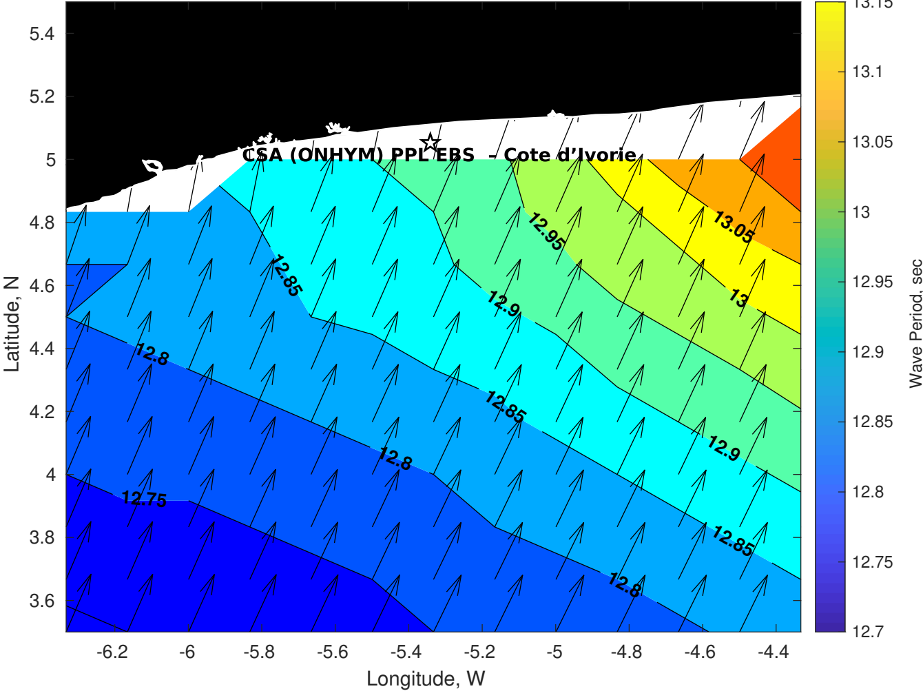
Wave Period (sec) for CSA (ONHYM) PPL EBS - Cote d'Ivoire at 19-Aug-2025 09:00:00
