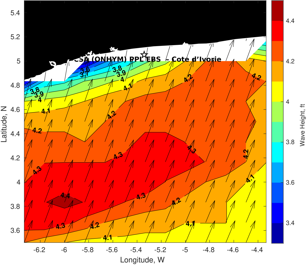
Wave Height (ft) for CSA (ONHYM) PPL EBS - Cote d'Ivoire at 19-Aug-2025 09:00:00
