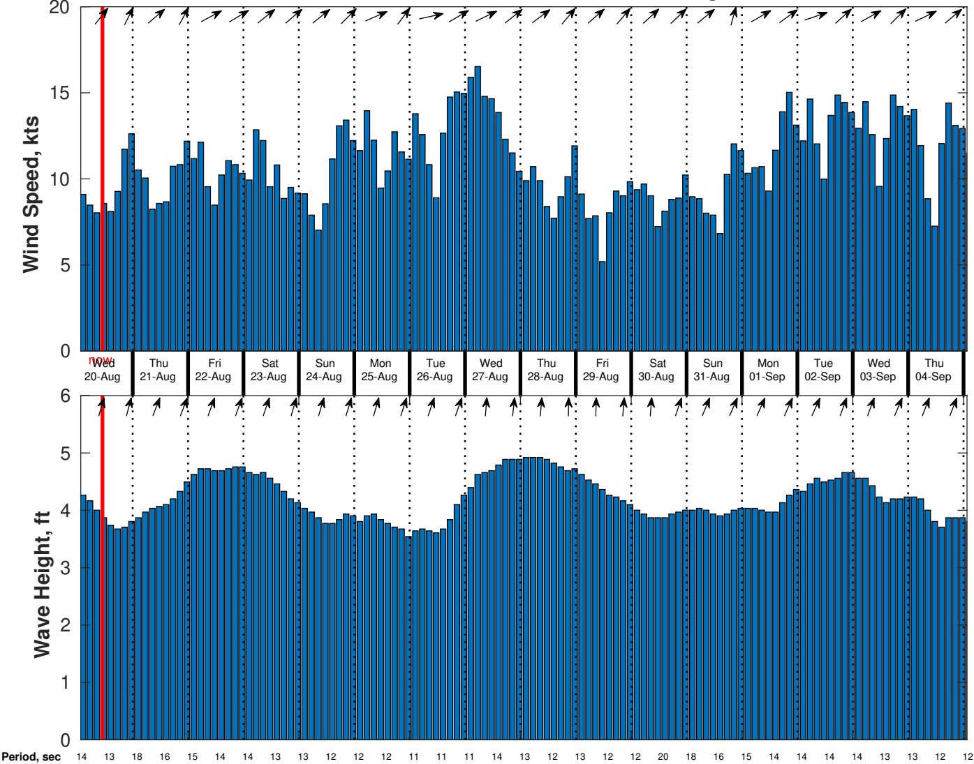
Wind & Wave Forecast for CSA (ONHYM) PPL EBS - Cote d'Ivoire from 19-Aug-2025 01:00:00 to 04-Sep-2025 01:00:00
