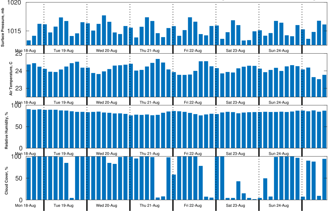
Met Forecast for CSA (ONHYM) PPL EBS - Cote d'Ivoire from 18-Aug-2025 12:00:00 to 25-Aug-2025 12:00:00
