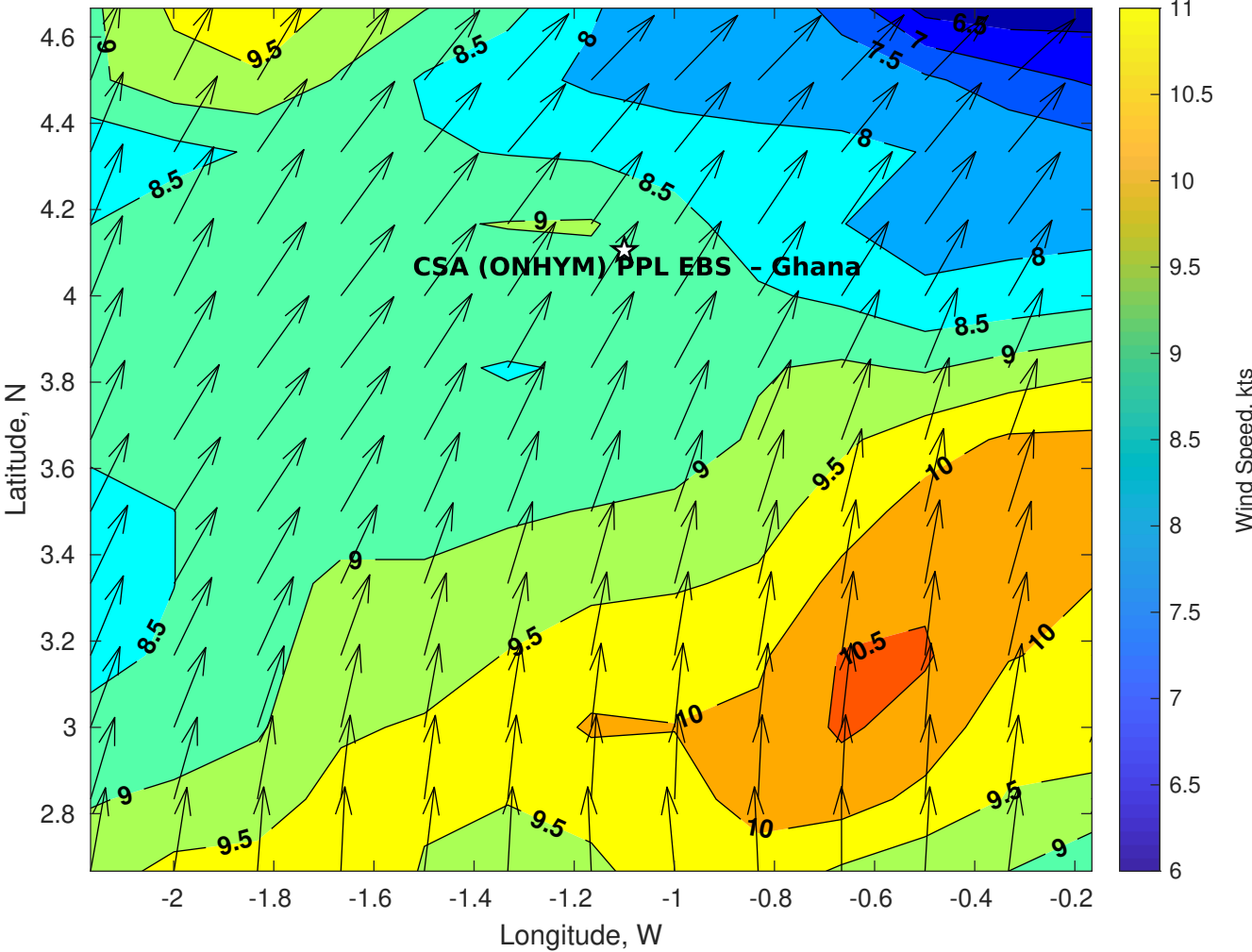
Winds (kts) for CSA (ONHYM) PPL EBS - Ghana at 19-Aug-2025 09:00:00
