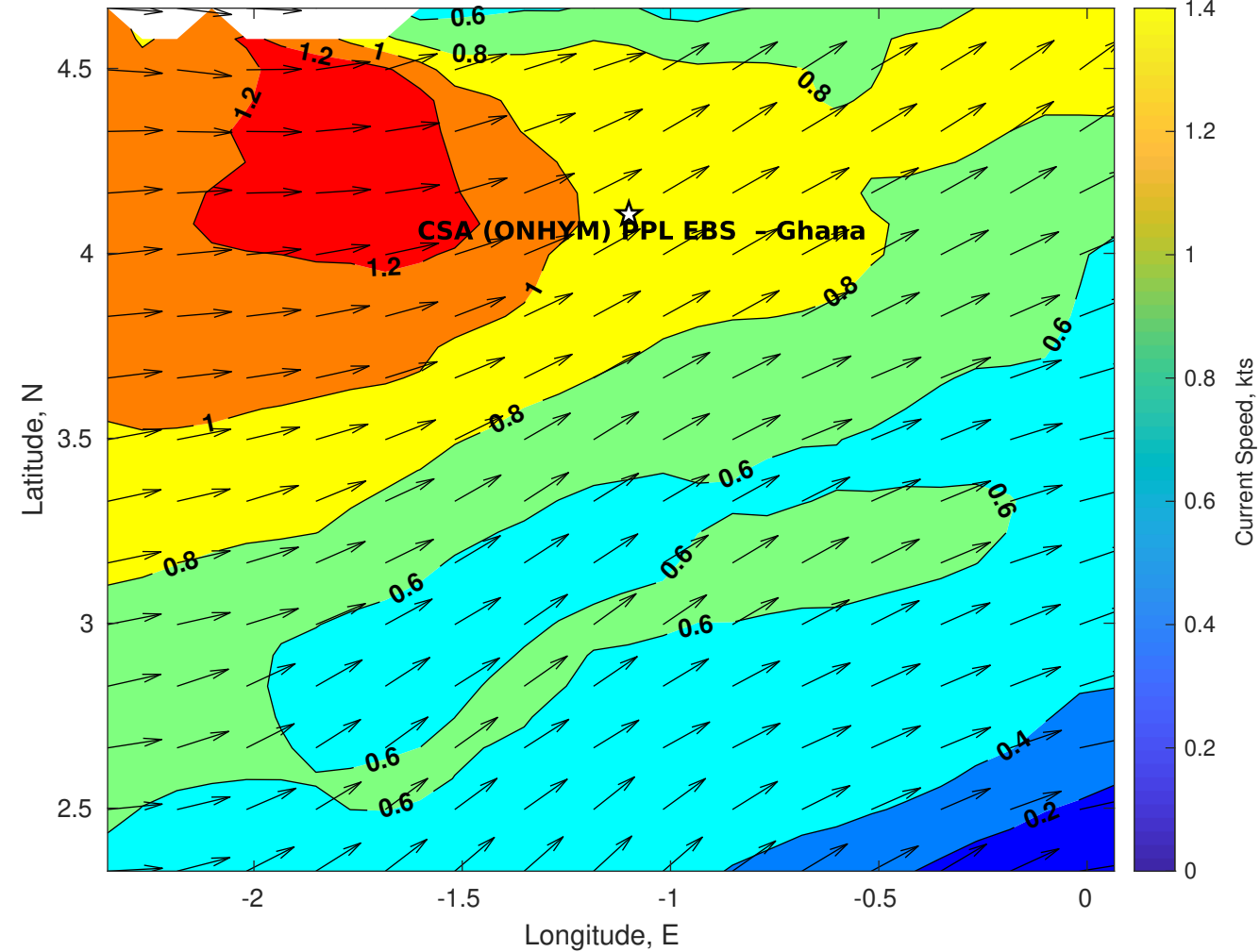
Surface Currents for CSA (ONHYM) PPL EBS - Ghana at 18-Aug-2025 00:00:00
