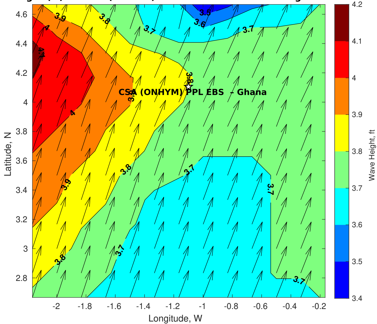
Wave Height (ft) for CSA (ONHYM) PPL EBS - Ghana at 19-Aug-2025 09:00:00
