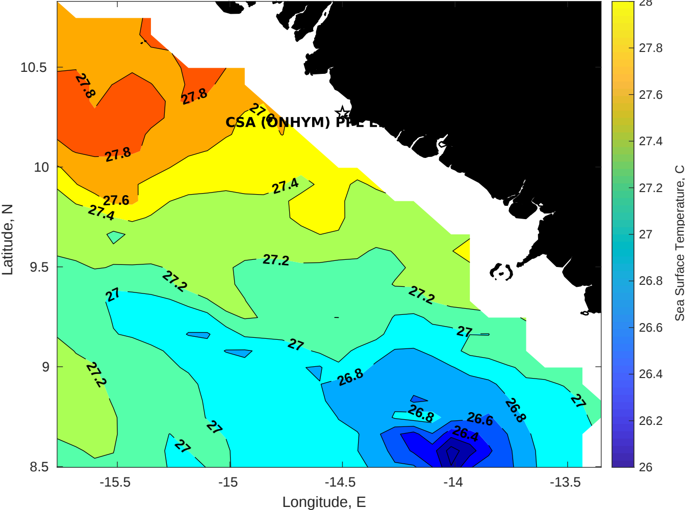
SST for CSA (ONHYM) PPL EBS - Guinea at 18-Aug-2025 00:00:00
