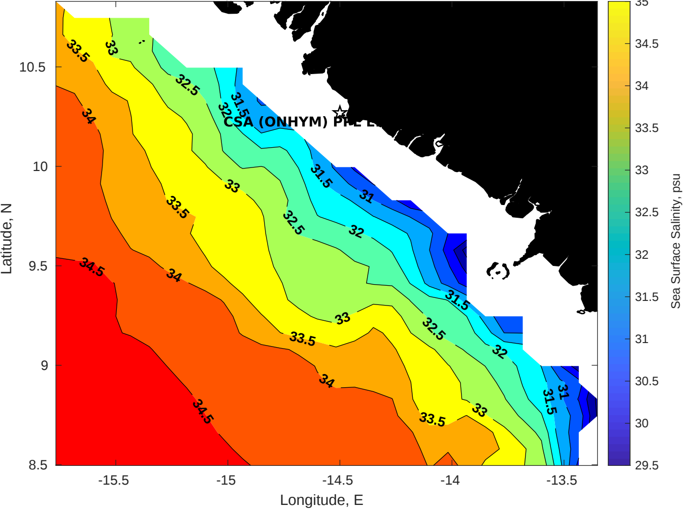
Surface Salinity for CSA (ONHYM) PPL EBS - Guinea at 18-Aug-2025 00:00:00
