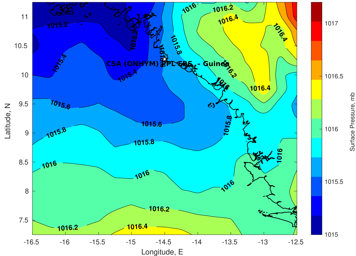
Surface Pressure (mb) for CSA (ONHYM) PPL EBS - Guinea at 19-Aug-2025 00:00:00
