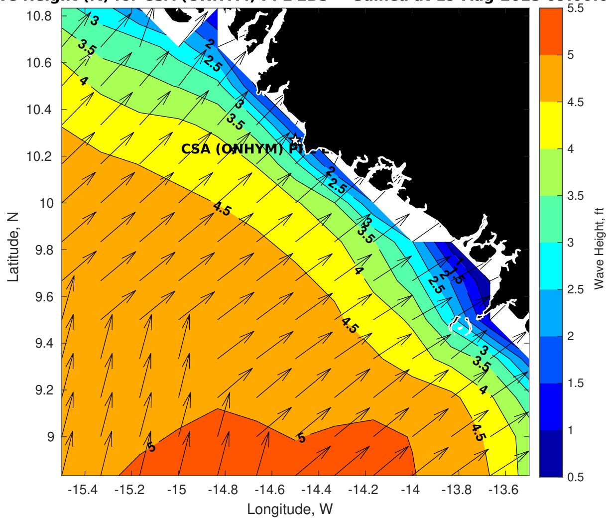
Wave Height (ft) for CSA (ONHYM) PPL EBS - Guinea at 19-Aug-2025 09:00:00
