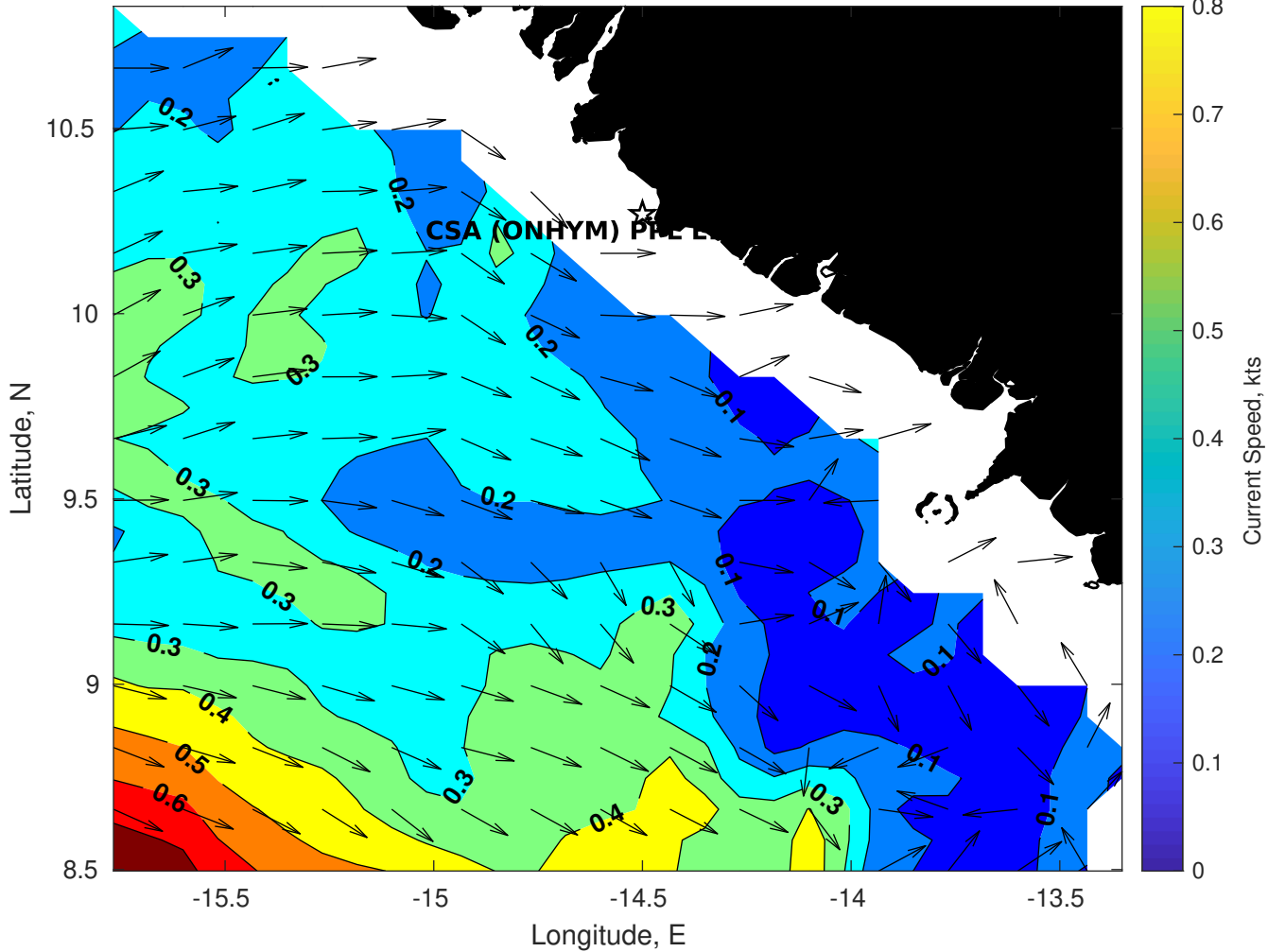
Surface Currents for CSA (ONHYM) PPL EBS - Guinea at 18-Aug-2025 00:00:00
