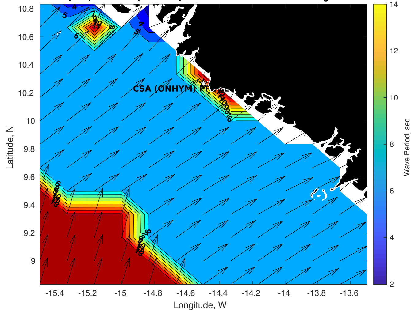
Wave Period (sec) for CSA (ONHYM) PPL EBS - Guinea at 19-Aug-2025 09:00:00
