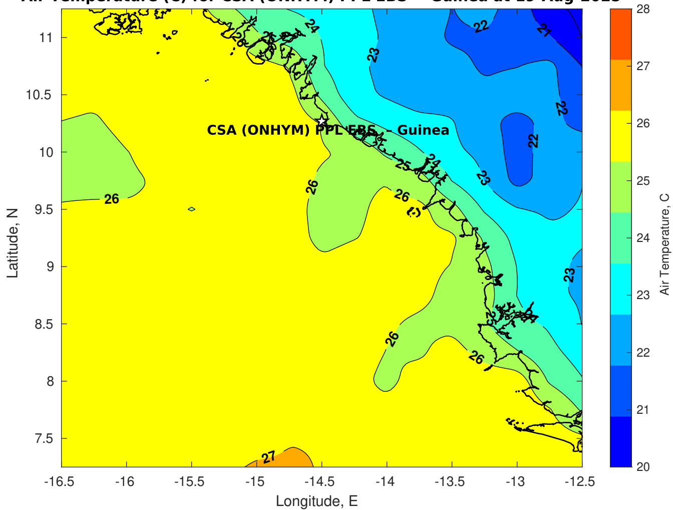
Air Temperature (C) for CSA (ONHYM) PPL EBS - Guinea at 19-Aug-2025
