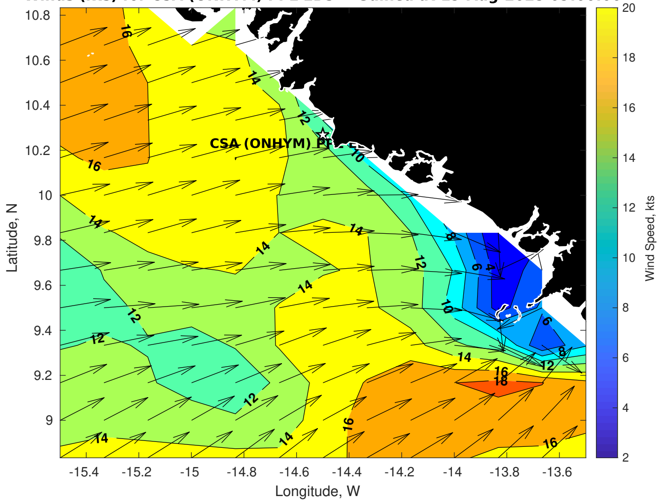
Winds (kts) for CSA (ONHYM) PPL EBS - Guinea at 19-Aug-2025 09:00:00
