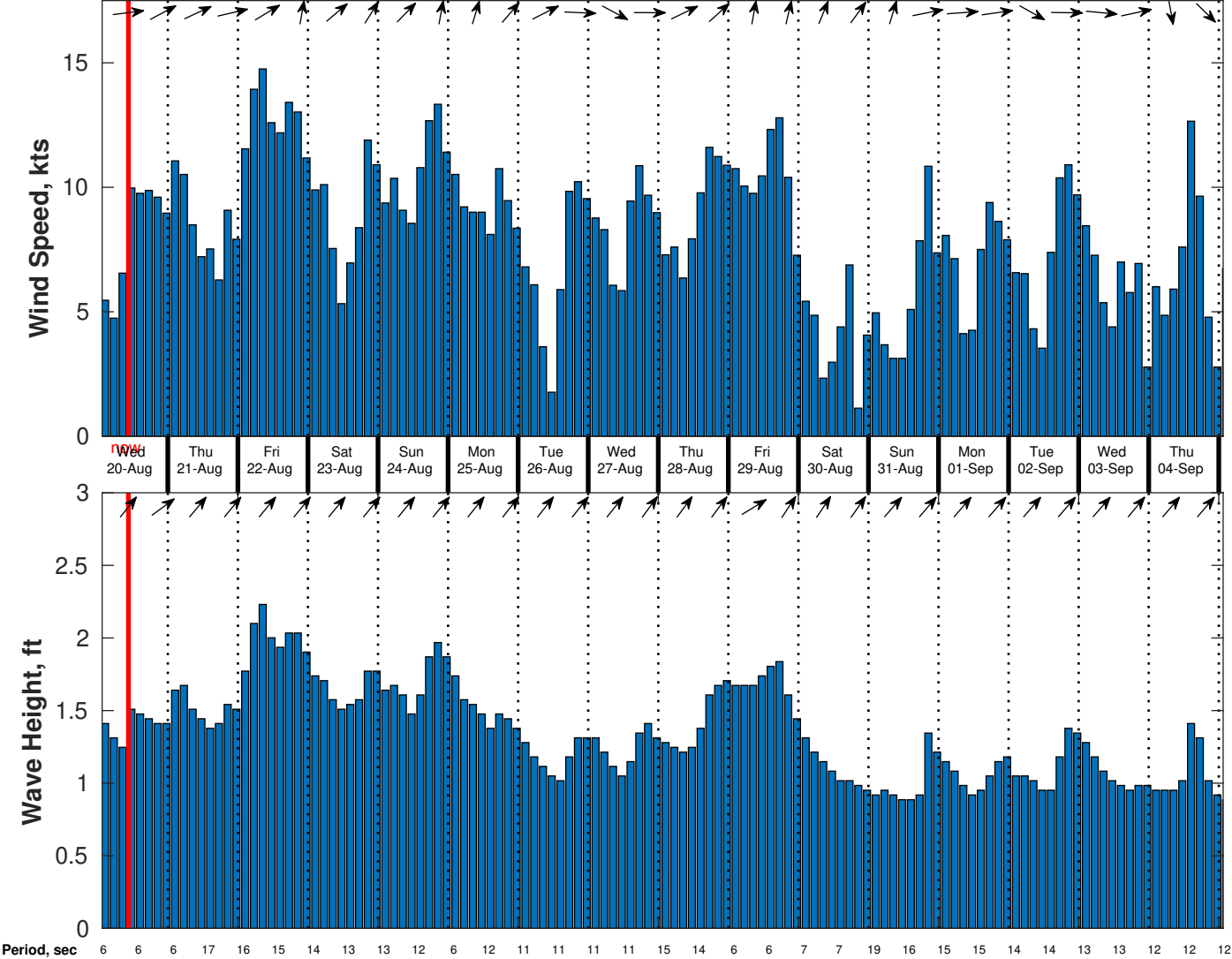
Wind & Wave Forecast for CSA (ONHYM) PPL EBS - Guinea from 19-Aug-2025 01:00:00 to 04-Sep-2025 01:00:00
