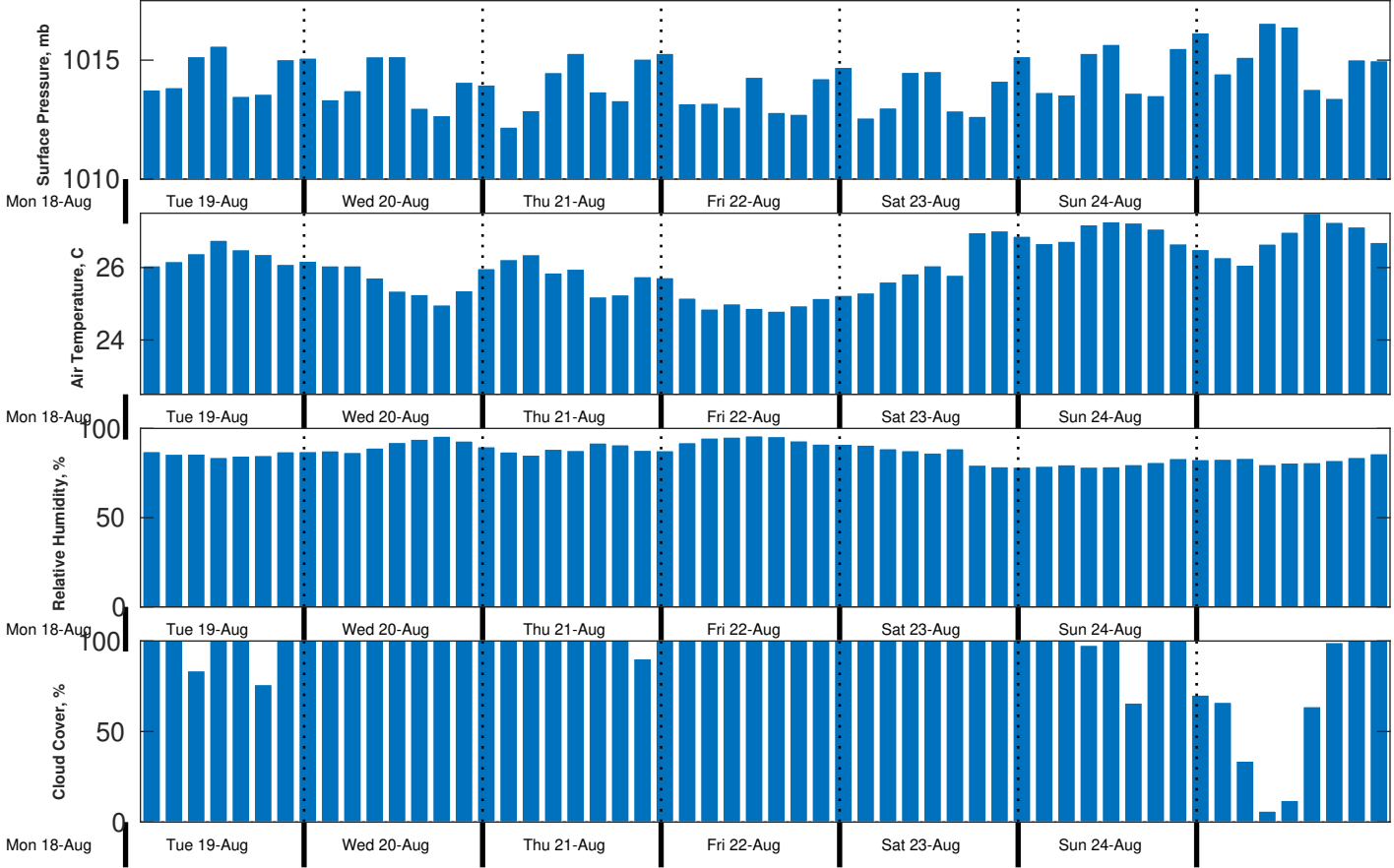
Met Forecast for CSA (ONHYM) PPL EBS - Guinea from 19-Aug-2025 00:00:00 to 26-Aug-2025 00:00:00
