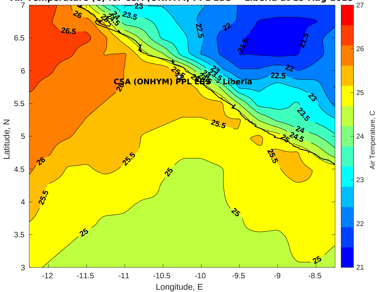
Air Temperature (C) for CSA (ONHYM) PPL EBS - Liberia at 19-Aug-2025
