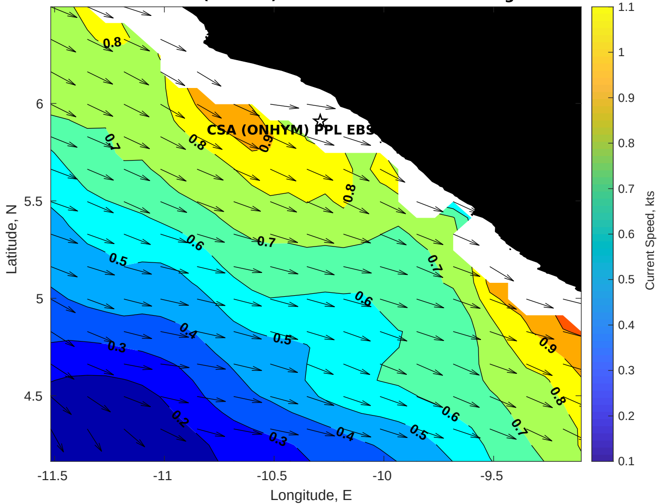
Surface Currents for CSA (ONHYM) PPL EBS - Liberia at 18-Aug-2025 00:00:00
