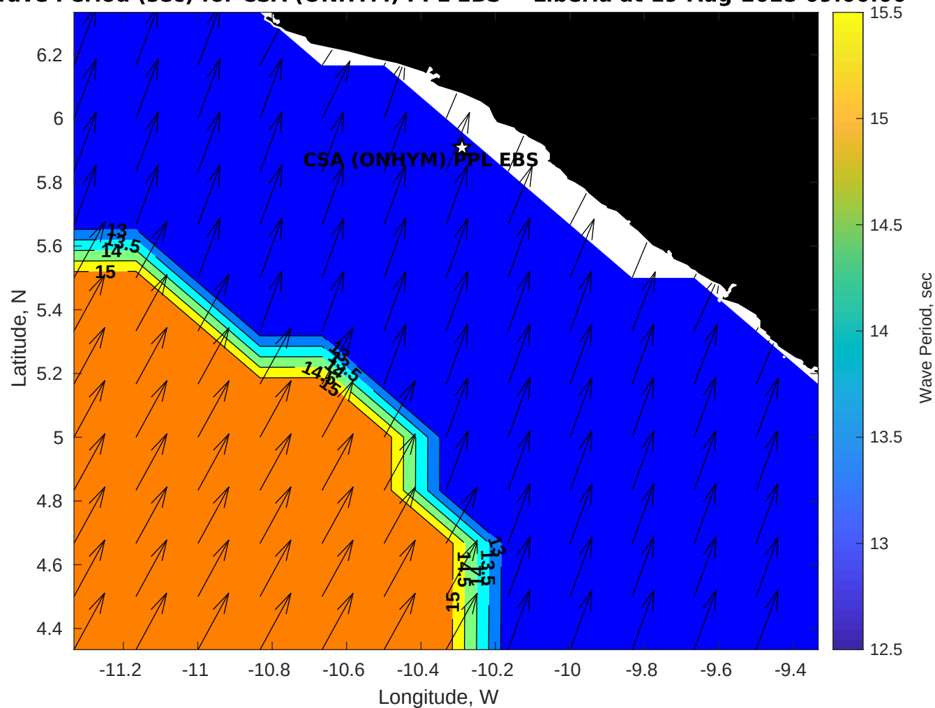
Wave Period (sec) for CSA (ONHYM) PPL EBS - Liberia at 19-Aug-2025 09:00:00
