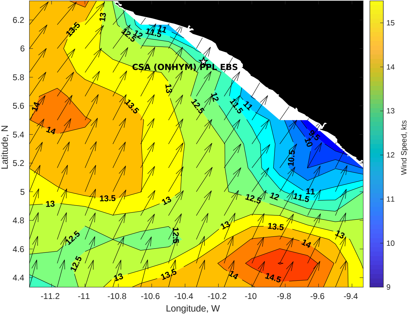
Winds (kts) for CSA (ONHYM) PPL EBS - Liberia at 19-Aug-2025 09:00:00
