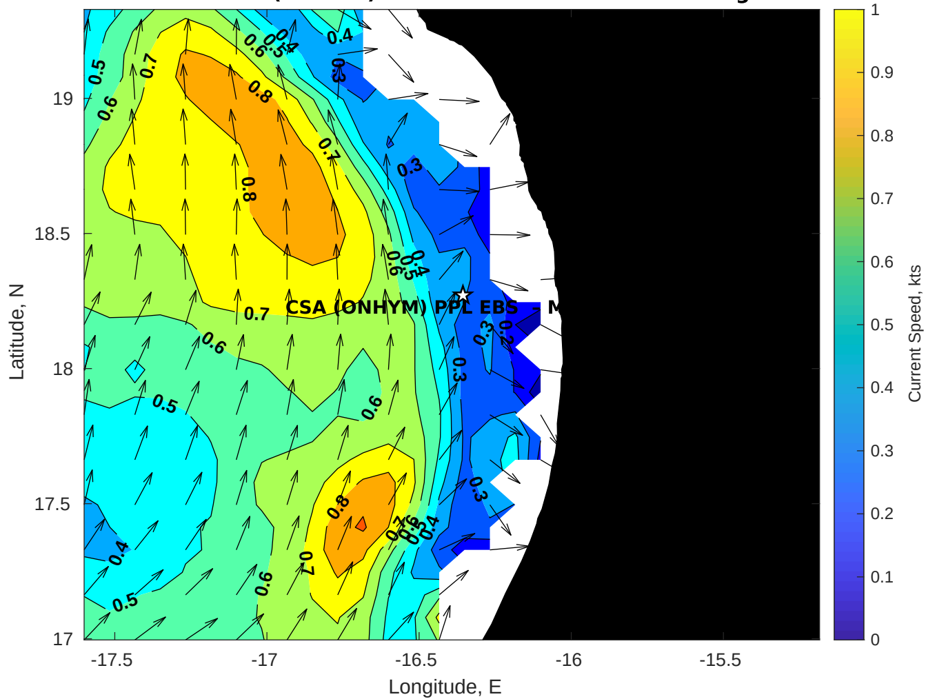
Surface Currents for CSA (ONHYM) PPL EBS - Mauritania at 18-Aug-2025 00:00:00
