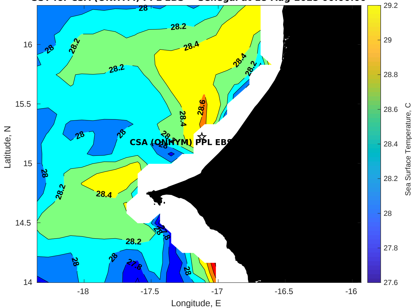
SST for CSA (ONHYM) PPL EBS - Senegal at 18-Aug-2025 00:00:00
