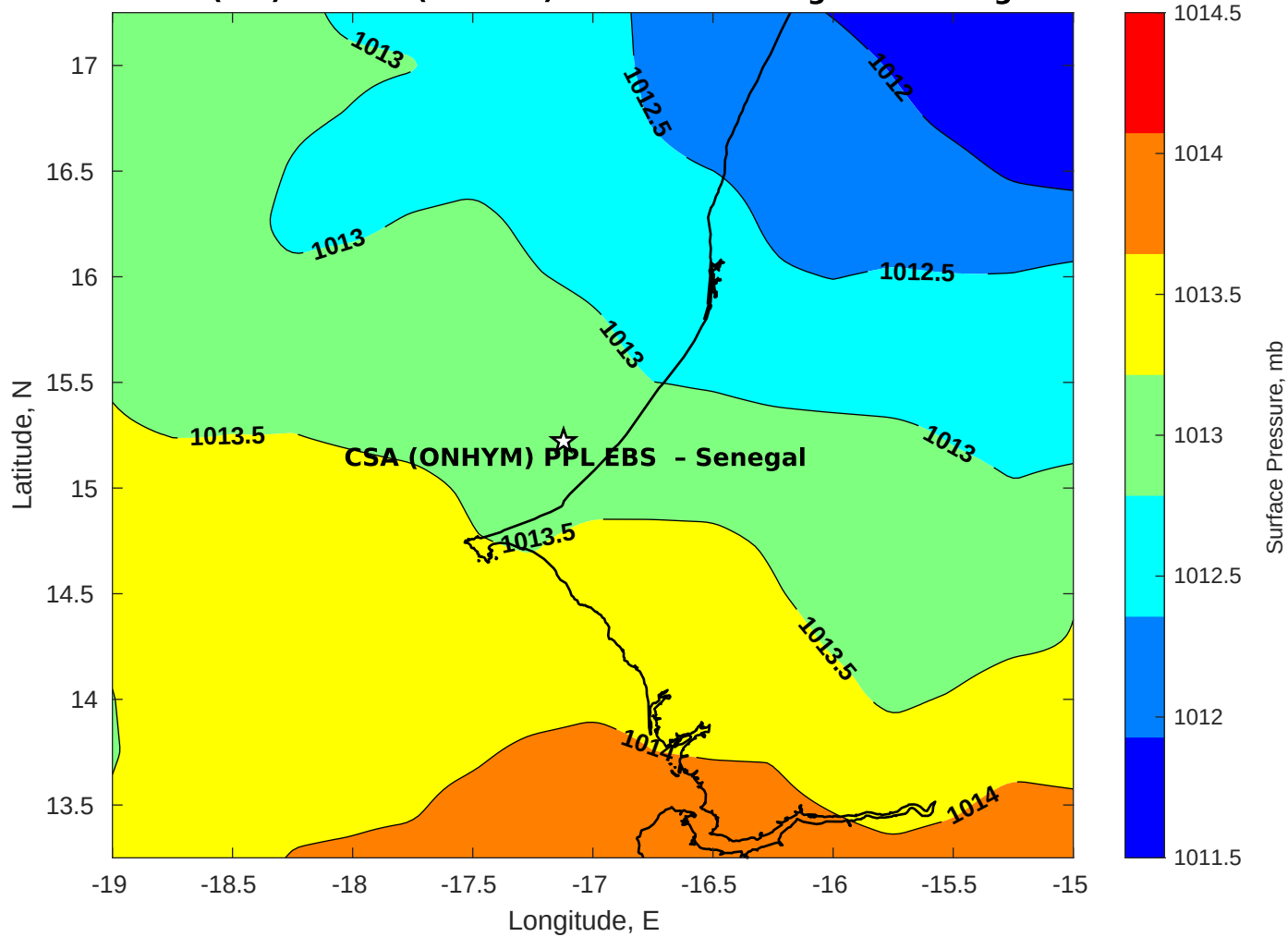
Surface Pressure (mb) for CSA (ONHYM) PPL EBS - Senegal at 20-Aug-2025 00:00:00
