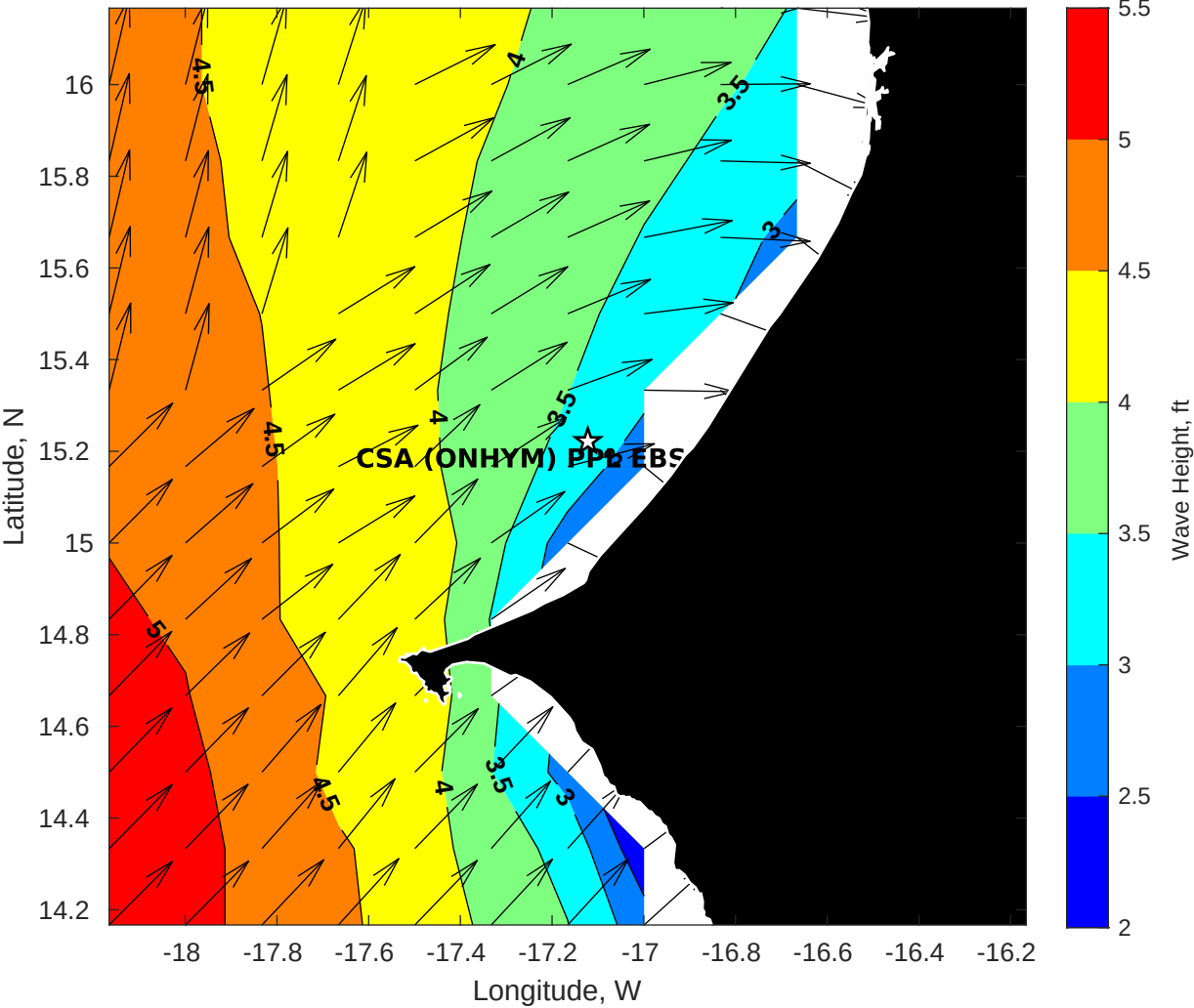
Wave Height (ft) for CSA (ONHYM) PPL EBS - Senegal at 19-Aug-2025 09:00:00
