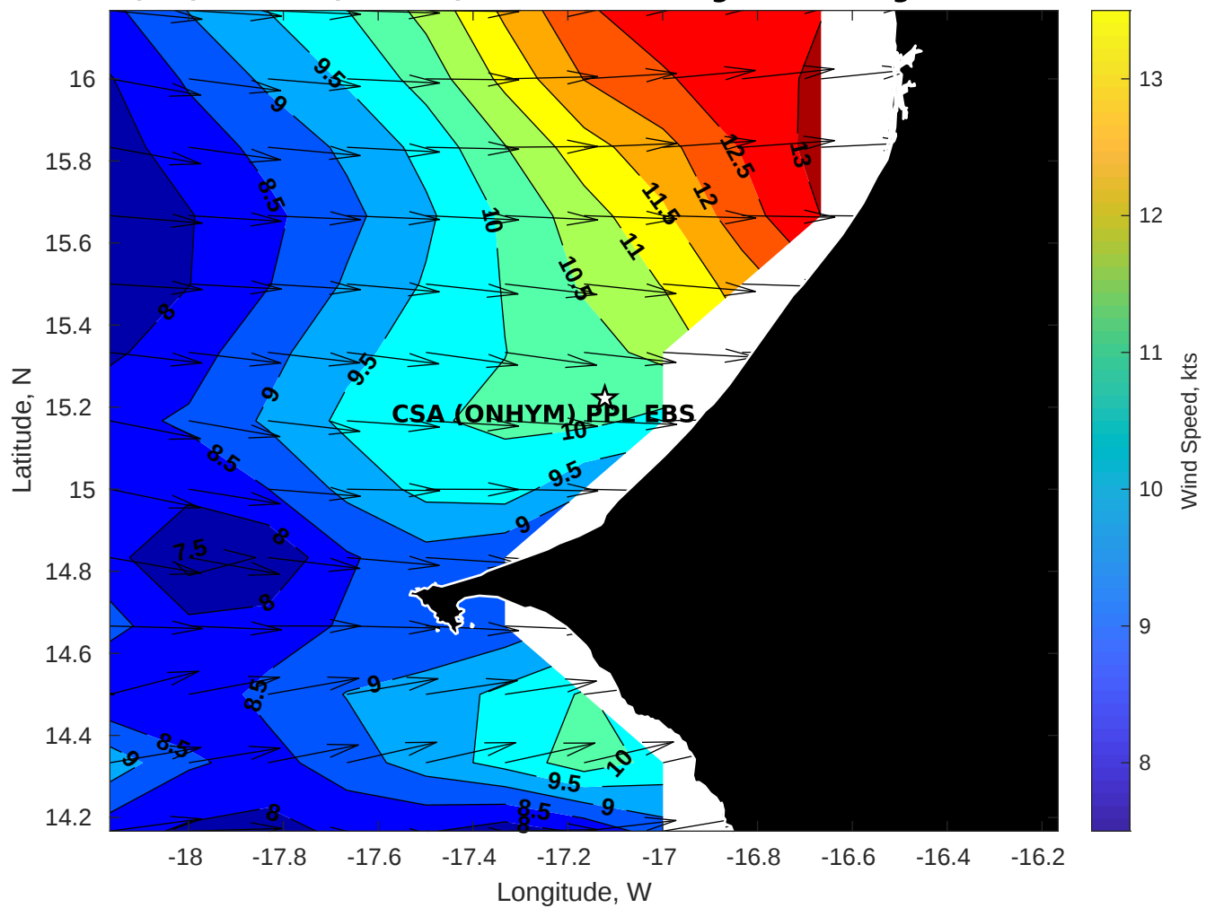
Winds (kts) for CSA (ONHYM) PPL EBS - Senegal at 19-Aug-2025 09:00:00
