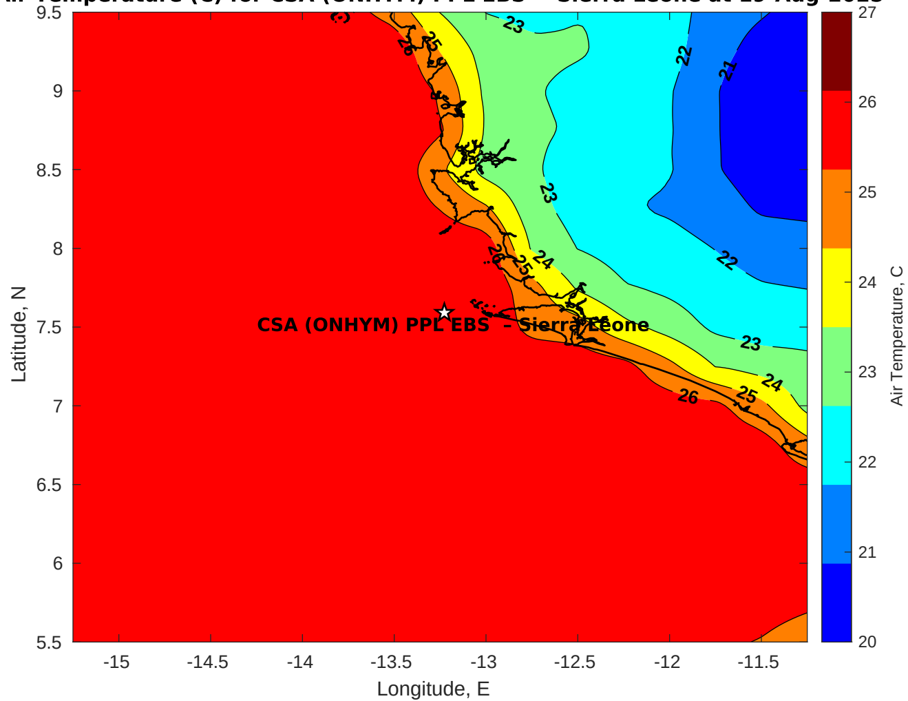
Air Temperature (C) for CSA (ONHYM) PPL EBS - Sierra Leone at 19-Aug-2025
