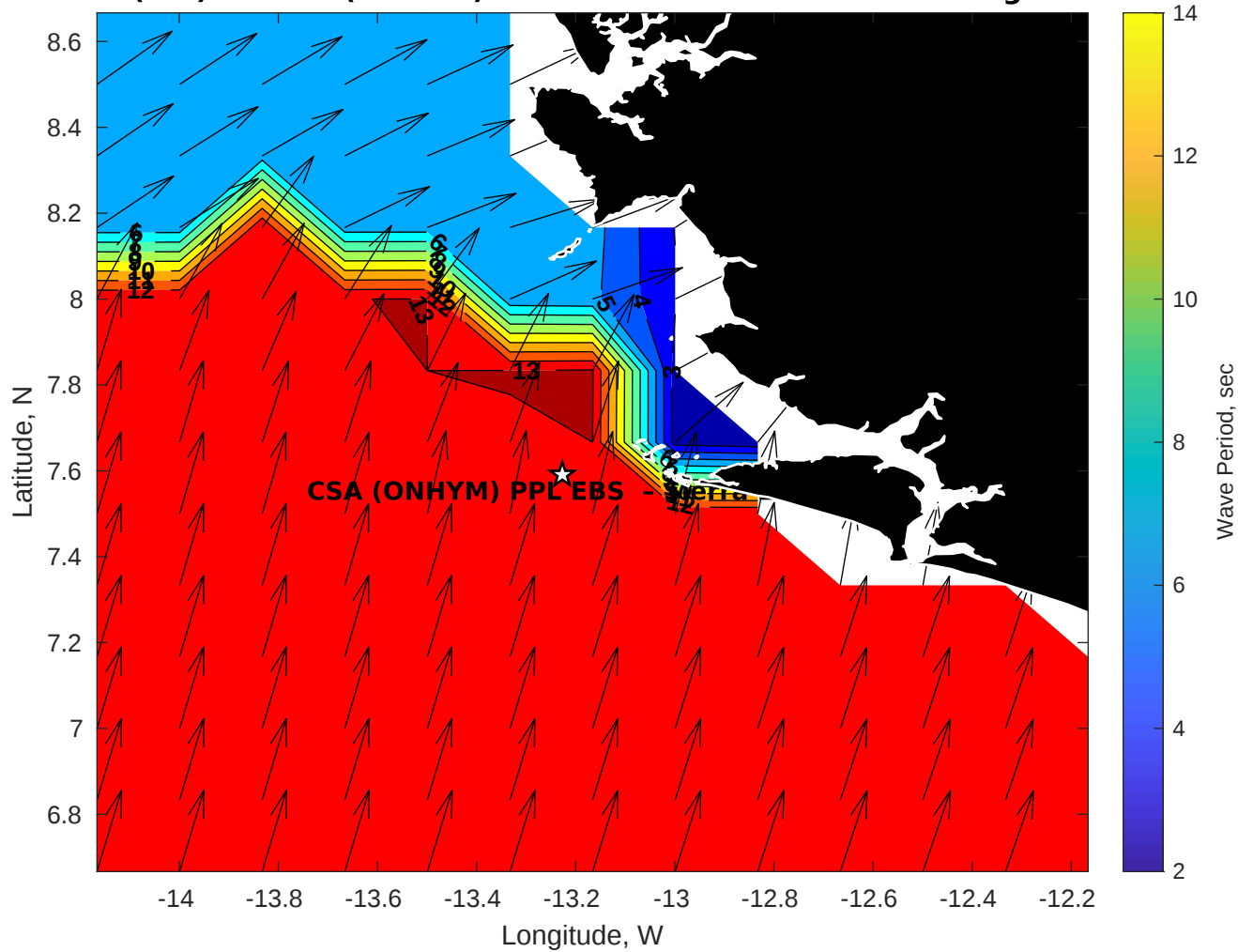
Wave Period (sec) for CSA (ONHYM) PPL EBS - Sierra Leone at 19-Aug-2025 09:00:00
