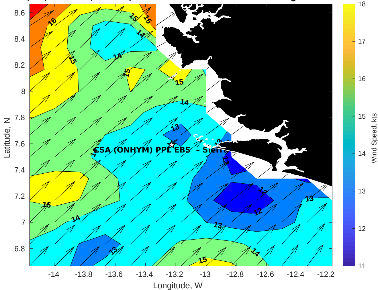
Winds (kts) for CSA (ONHYM) PPL EBS - Sierra Leone at 19-Aug-2025 09:00:00
