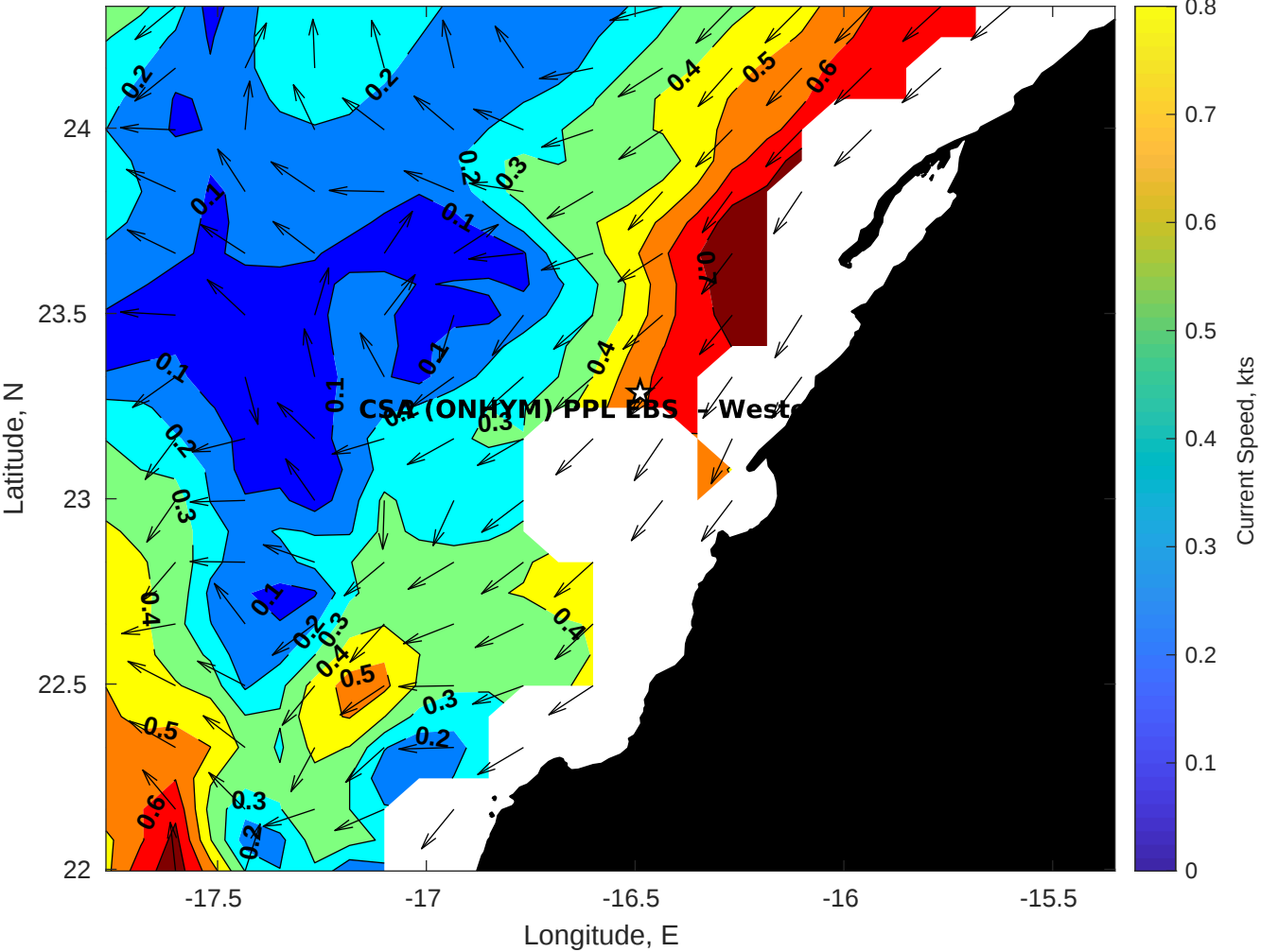
Surface Currents for CSA (ONHYM) PPL EBS - Western Sahara at 18-Aug-2025 00:00:00
