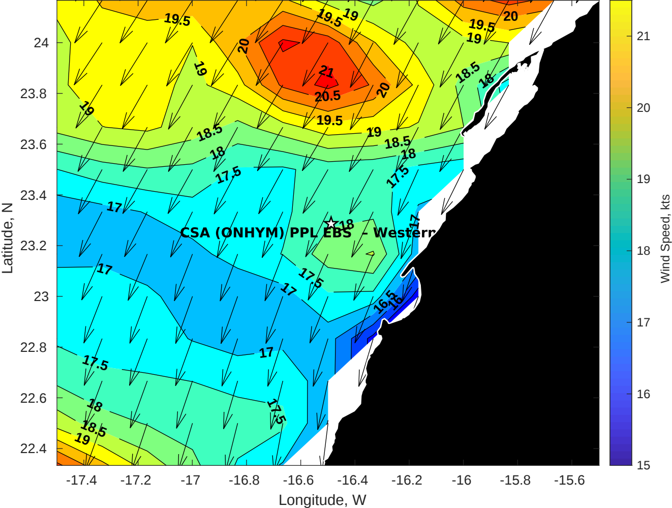
Winds (kts) for CSA (ONHYM) PPL EBS - Western Sahara at 19-Aug-2025 09:00:00
