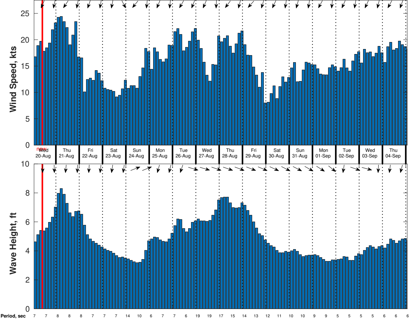
Wind & Wave Forecast for CSA (ONHYM) PPL EBS - Western Sahara from 19-Aug-2025 01:00:00 to 04-Sep-2025 01:00:00
