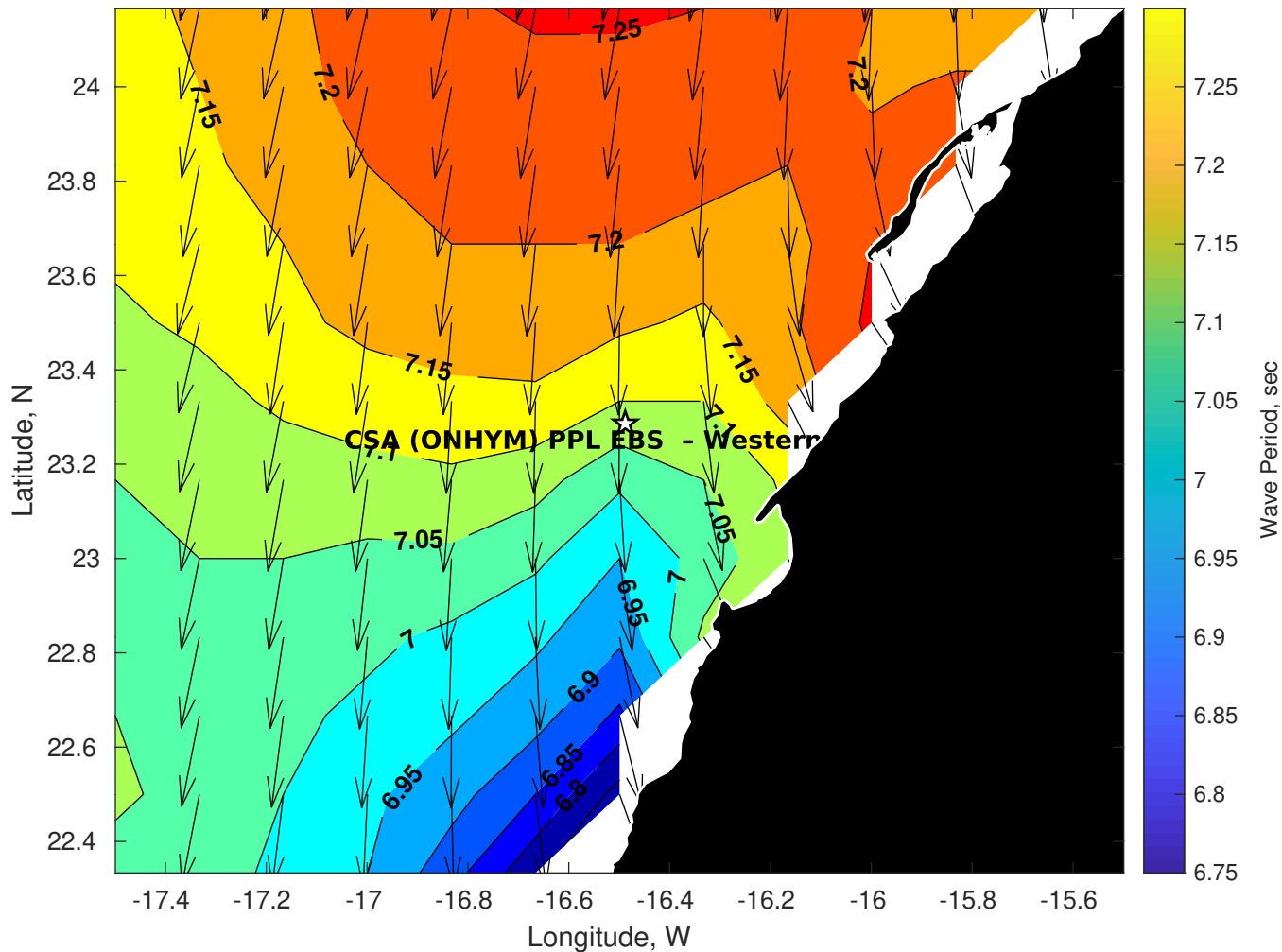
Wave Period (sec) for CSA (ONHYM) PPL EBS - Western Sahara at 19-Aug-2025 09:00:00
