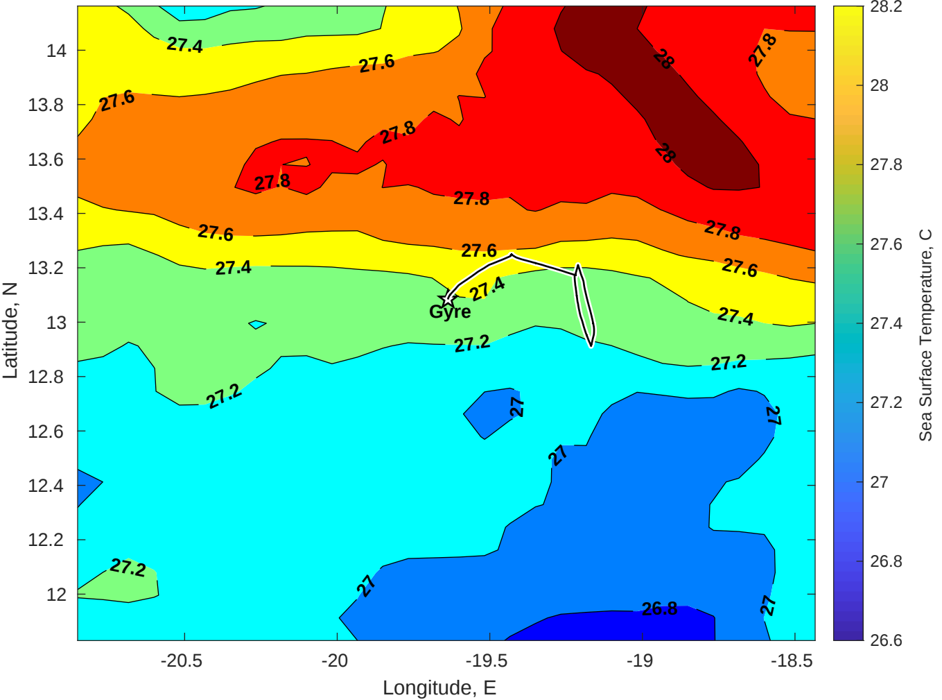
SST for Gyre at 18-Aug-2025 00:00:00
