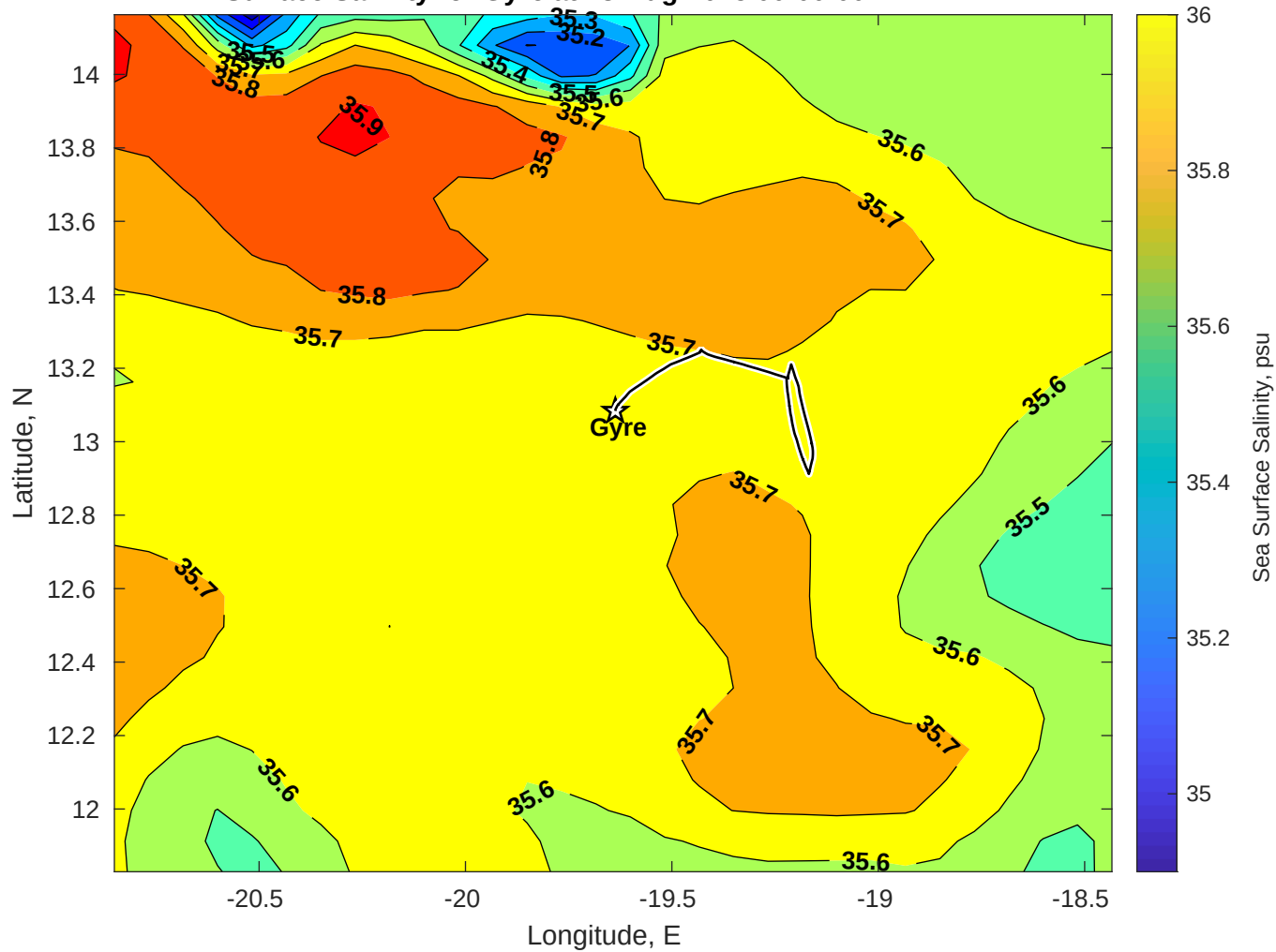
Surface Salinity for Gyre at 18-Aug-2025 00:00:00
